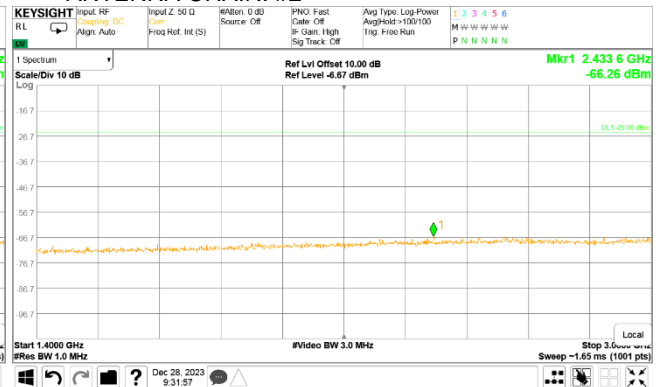
Plot 7.5.39 Spurious emission measurements in 1400 - 3000 MHz range at high carrier frequency
