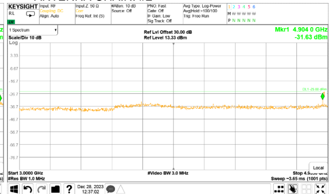
Plot 7.5.14 Spurious emission measurements in 3000 - 4935 range at mid carrier frequency
