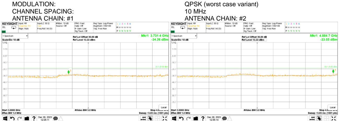
Plot 7.5.15 Spurious emission measurements in 3000 - 4935 range at high carrier frequency
