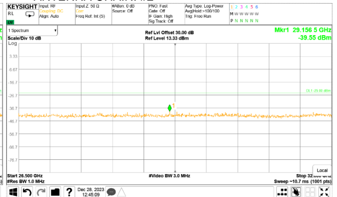
Plot 7.5.24 Spurious emission measurements in 26.5 - 32 GHz range at high carrier frequency
