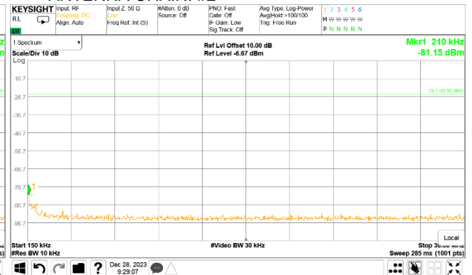
Plot 7.5.33 Spurious emission measurements in 150 kHz – 30 MHz range at high carrier frequency
