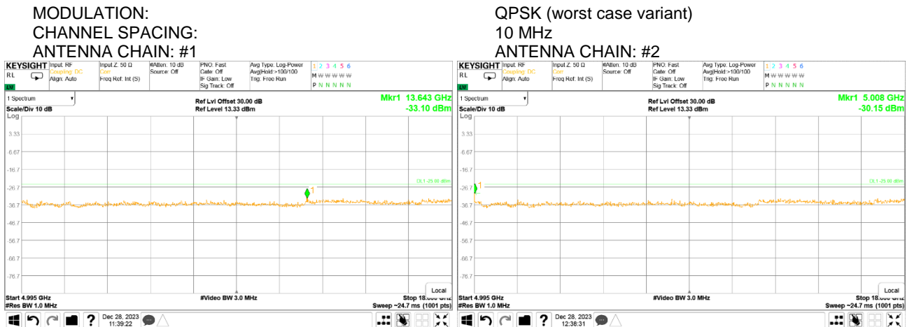
Plot 7.5.16 Spurious emission measurements in 4995 - 18000 MHz range at low carrier frequency
