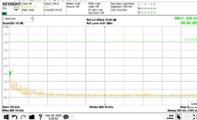
Plot 7.5.33 Spurious emission measurements in 150 kHz – 30 MHz range at high carrier frequency
