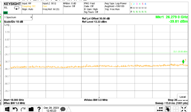
Plot 7.5.20 Spurious emission measurements in 18 – 26.5 GHz range at mid carrier frequency
