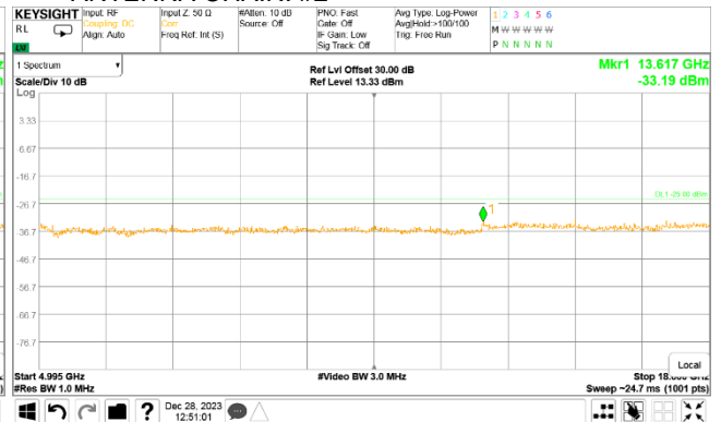
Plot 7.5.18 Spurious emission measurements in 4995 - 18000 MHz range at high carrier frequency
