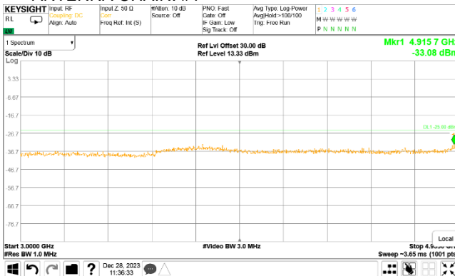
Plot 7.5.14 Spurious emission measurements in 3000 - 4935 range at mid carrier frequency
