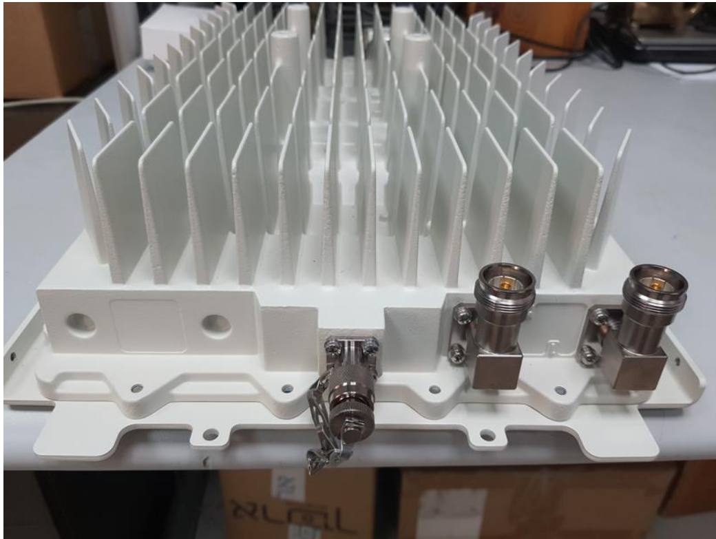
Photograph No.4 “AirSpeed 1900, 4.94 – 4.99GHz (n79)” base station side panel view (Antenna connectors side)
