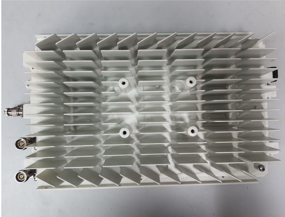
Photograph No.2 “AirSpeed 1900, 4.94 – 4.99GHz (n79)” base station rear panel view
