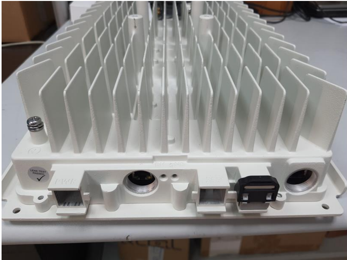
Photograph No.3 “AirSpeed 1900, 4.94 – 4.99GHz (n79)” base station side panel view (Cables connection side)
