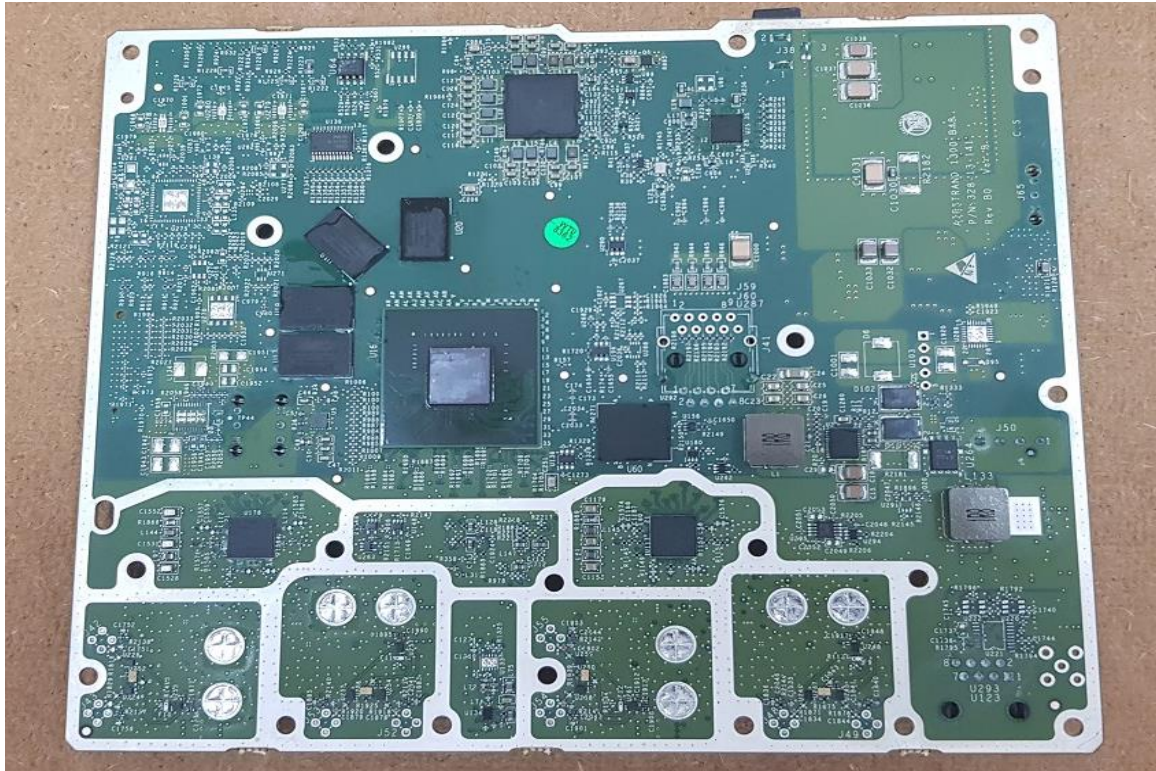
Photograph No.7 eNB card_3 view
