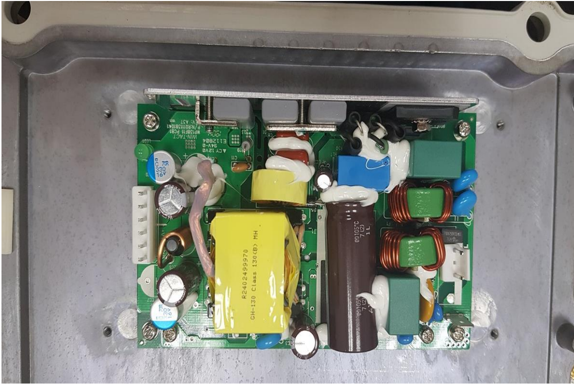
Photograph No.10 PS card view
