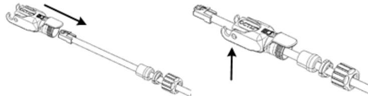
Figure 32: Insert Housing onto Cable
