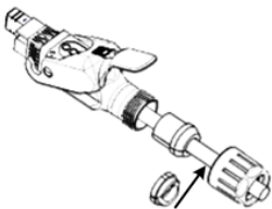
Figure 49: Place Tightening Cone on Split Gland
