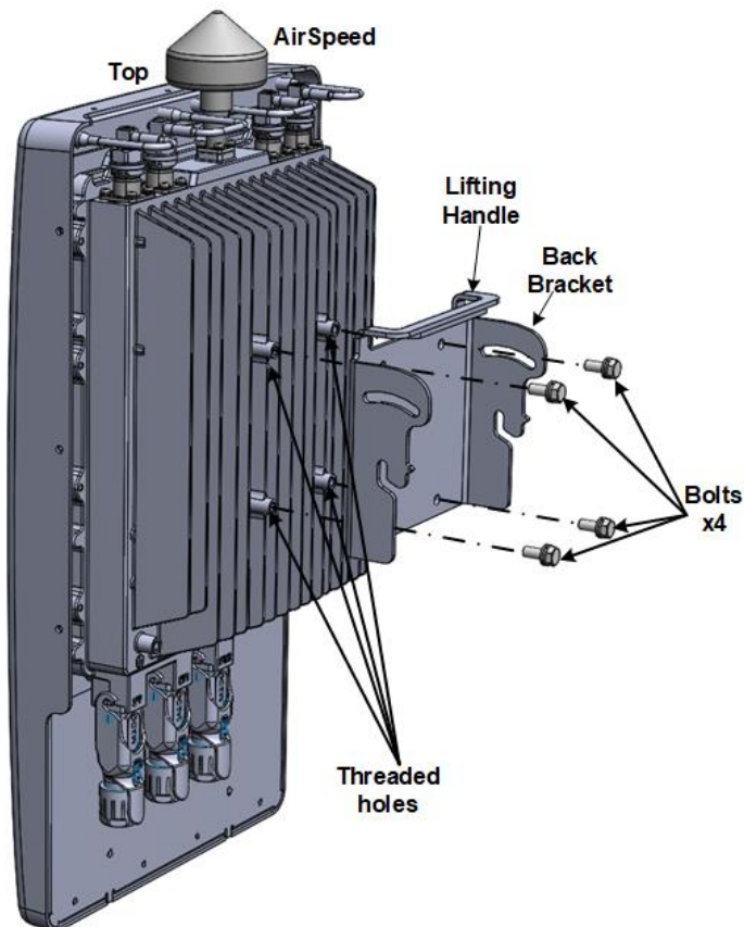
Figure 6: Back Bracket Assembly
