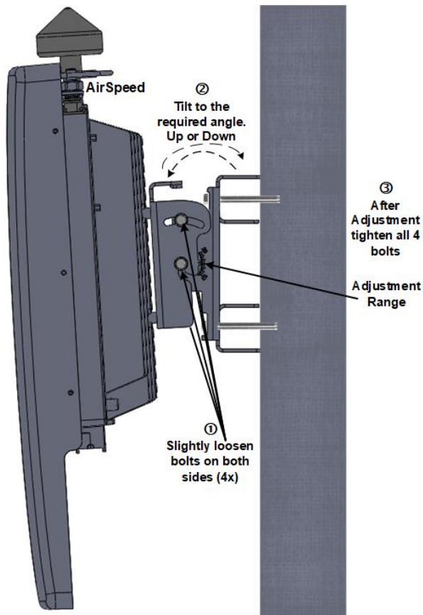
Figure 11: Tilt Adjustment
