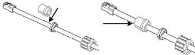
Figure 31: Insert Rubber Gland on Cable
