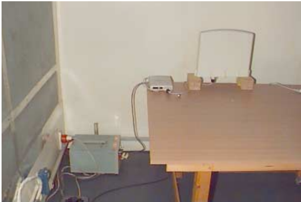
Photograph No.5 Conducted emission measurement on AC line setup, BSR
