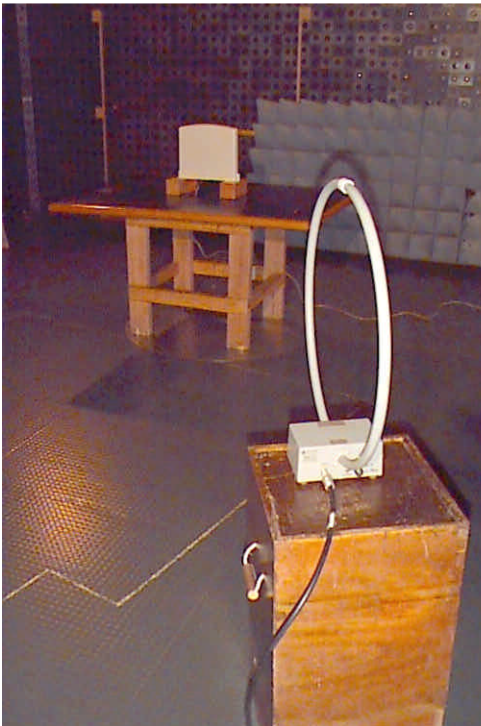
Photograph No.1 Spurious emissions measurement setup in the anechoic chamber with loop antenna
