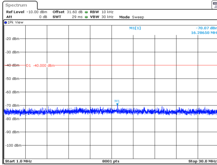
Plot 7.6.8 Spurious emission measurements in 1- 30.0 MHz range at mid carrier frequency
