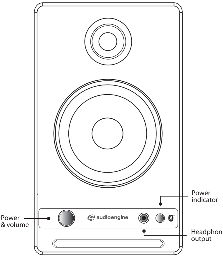
HD4 powered (left) speaker
