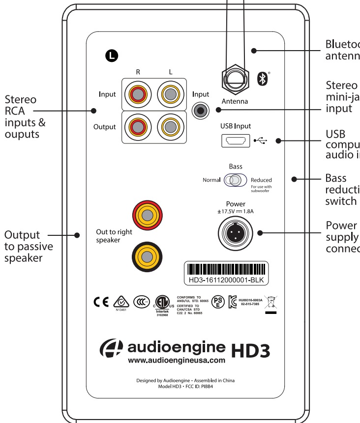
HD3 powered (left) speaker - rear panel
