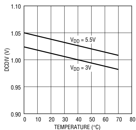
DCDIV Trip Point vs Temperature
