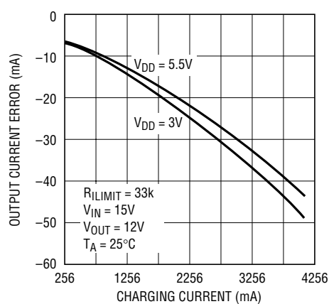
Programmed Current Accuracy
