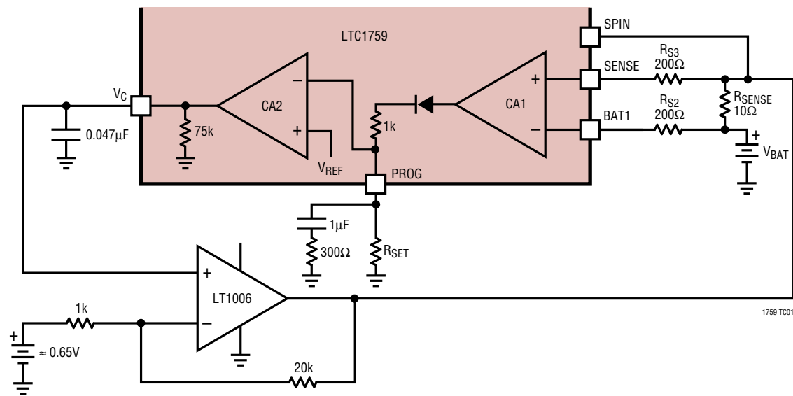
Test Circuit 1
