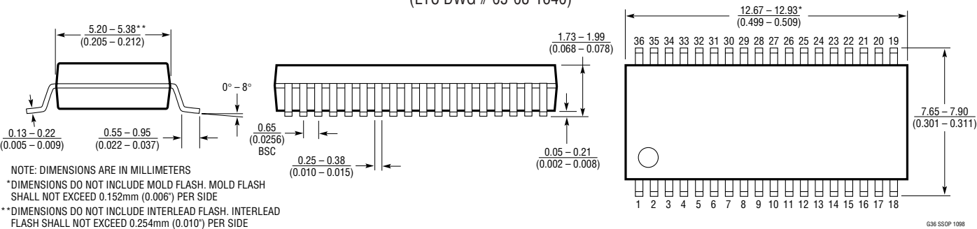
G Package 36-Lead Plastic SSOP (0.209) (LTC DWG # 05-08-1640)
