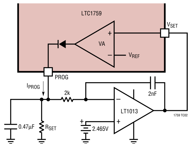
Test Circuit 2
