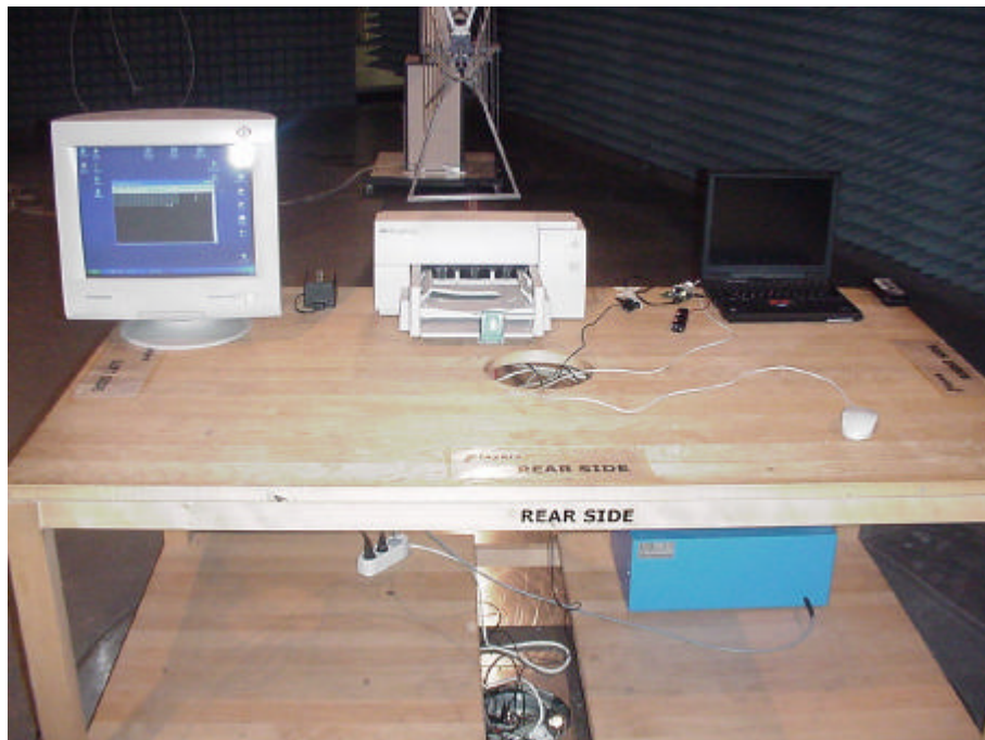
Picture 2 : Setup for radiated emission measurement (front view)
