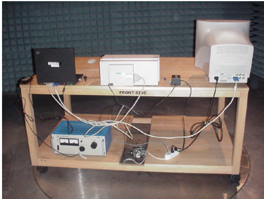
Picture 3 : Setup for radiated emission measurement (rear view)
