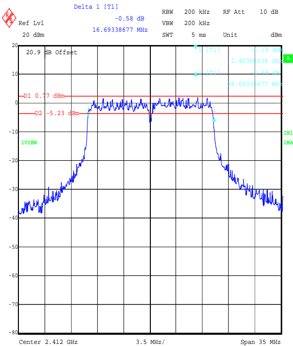
Title: Ezurio 2.4 GHz WLAN module, FCC P15.247 6 dB Bandwidth Comment A: 48271JD05 Bottom Channel, 64QAM OFDM. Date: 5.SEP.2006 16:31:12
