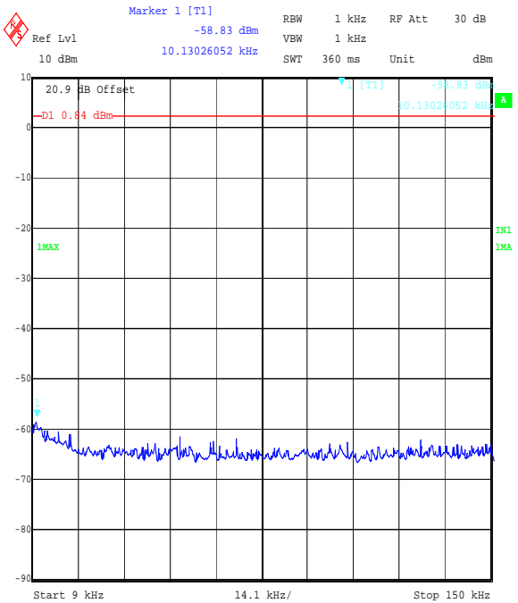
Title: EZURIO 2.4 GHz WLAN Module, FCC Part 15.247 Cond. Emissions Comment A: 48271JD05 Top Channel OFDM BPSK Date: 8.SEP.2006 16:47:44
