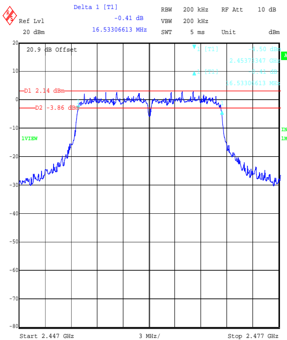
Title: EZURIO 2.4 GHz WLAN Module. FCC Part 15.247 6 dB Bandwidth Comment A: 48271JD05 Top Channel OFDM QPSK Date: 8.SEP.2006 15:56:56
