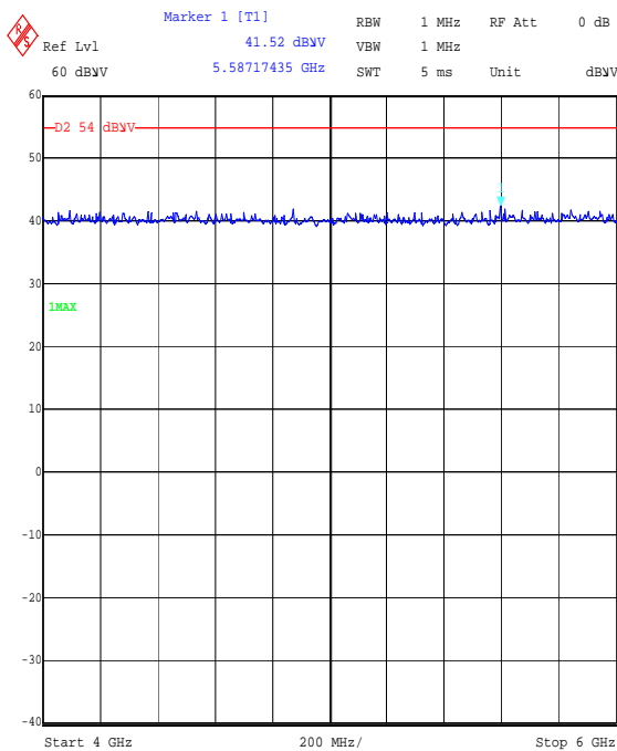
Title: Ezurio 2.4GHz WLAN FCC P15.247 Radiated Emissions Comment A: 48271JD05 RX mode Date: 7.SEP.2006 14:38:01
