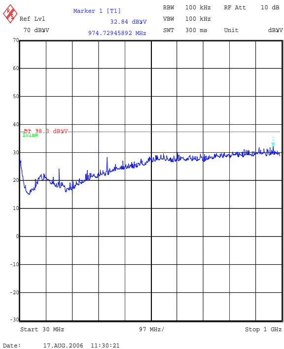
Pre-scan with 2 dBi antenna
