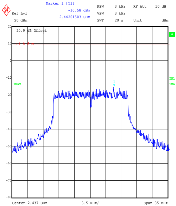
Title: Ezurio 2.4 GHz WLAN module, FCC P15.247 Spectral Density Comment A: 48271JD05 Middle Channel, BPSK OFDM. Date: 5.SEP.2006 14:23:06
