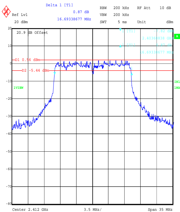
Title: Ezurio 2.4 GHz WLAN module, FCC P15.247 6 dB Bandwidth Comment A: 48271JD05 Bottom Channel, 16QAM OFDM. Date: 5.SEP.2006 16:32:19
