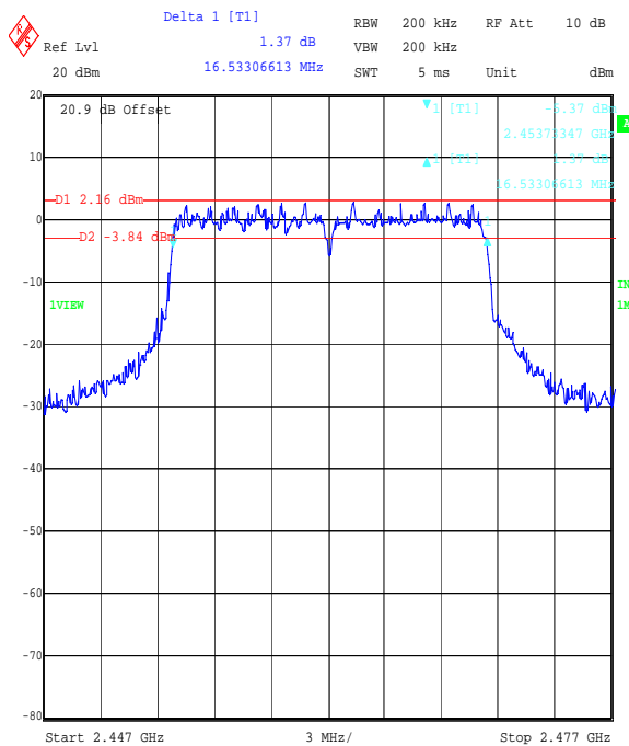
Title: EZURIO 2.4 GHz WLAN Module, FCC Part 15.247 6 dB Bandwidth Comment A: 48271JD05 Top Channel OFDM 16QAM Date: 8.SEP.2006 15:59:12
