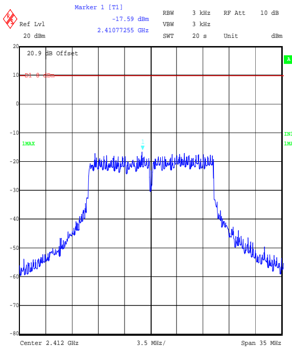
Title: Ezurio 2.4 GHz WLAN module, FCC P15.247 Spectral Density Comment A: 48271JD05 Bottom Channel, QPSK OFDM. Date: 5.SEP.2006 14:21:12
