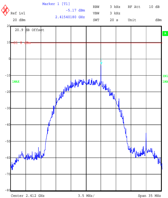
Title: Ezurio 2.4 GHz WLAN module, FCC P15.247 Spectral Density Comment A: 48271JD05 Bottom Channel, CCK DSSS. Date: 5.SEP.2006 14:14:52
