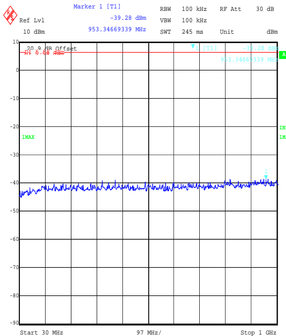
Title: EZURIO 2.4 GHz WLAN Module, FCC Part 15.247 Cond. Emissions Comment A: 48271JD05 Top Channel DSSS BPSK Date: 8.SEP.2006 17:04:00
