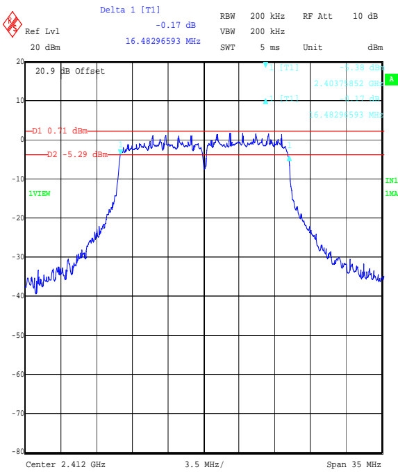
Title: Ezurio 2.4 GHz WLAN module. FCC P15.247 6 dB Bandwidth Comment A: 48271JD05 Bottom Channel, QPSK OFDM. Date: 5.SEP.2006 16:33:51
