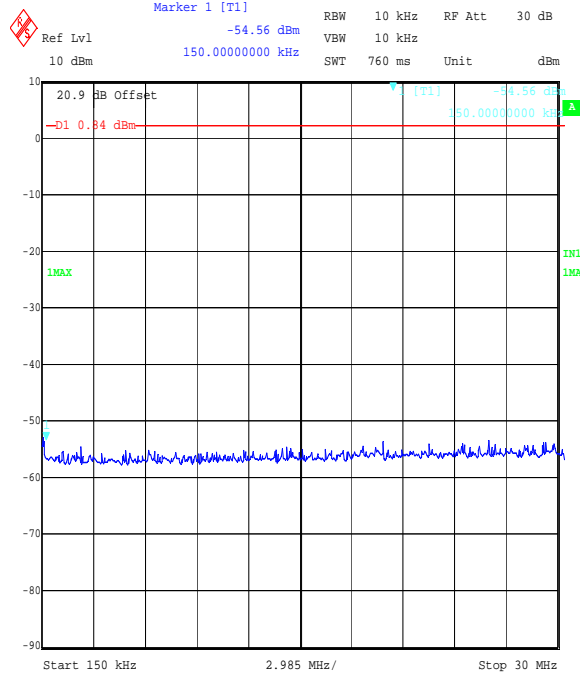
Title: EZURIO 2.4 GHz WLAN Module, FCC Part 15.247 Cond. Emissions Comment A: 48271JD05 Top Channel OFDM BPSK Date: 8.SEP.2006 16:50:13
