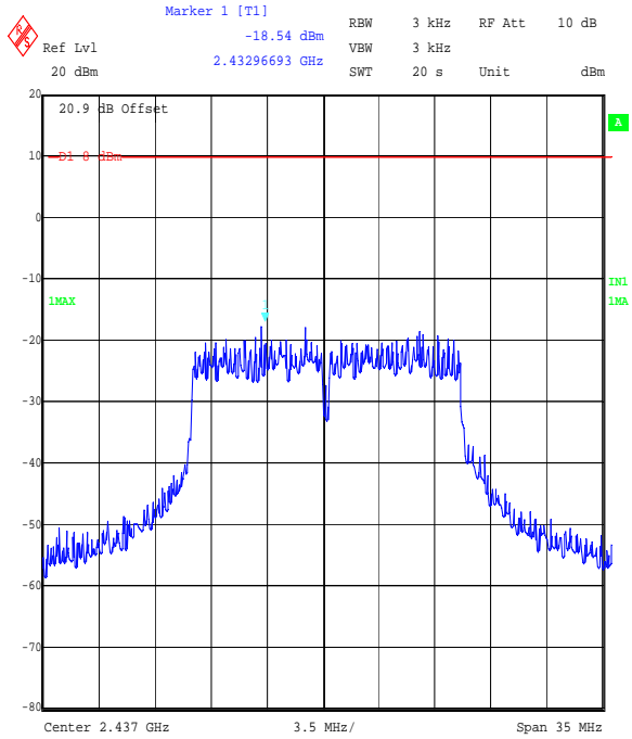
Title: Ezurio 2.4 GHz WLAN module, FCC P15.247 Spectral Density Comment A: 48271JD05 Middle Channel, 64QAM OFDM. Date: 5.SEP.2006 14:25:02
