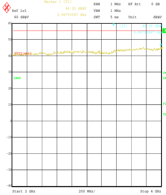
Title: Ezurio Test No 48271JD02 FCC Part 15.247 Comment A: Radiated Emissions Scans Rx Mode Date: 6.SEP.2006 16:09:22
