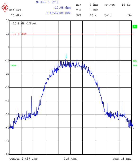
Title: Ezurio 2.4 GHz WLAN module, FCC P15.247 Spectral Density Comment A: 48271JD05 Middle Channel, QPSK DSSS. Date: 5.SEP.2006 14:27:13
