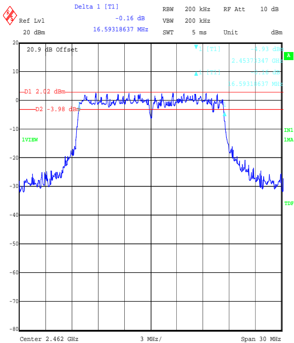
Title: EZURIO 2.4 GHz WLAN Module, FCC Part 15.247 6 dB Bandwidth Comment A: 48271JD05 Top Channel OFDM 64QAM Date: 8.SEP.2006 16:02:06
