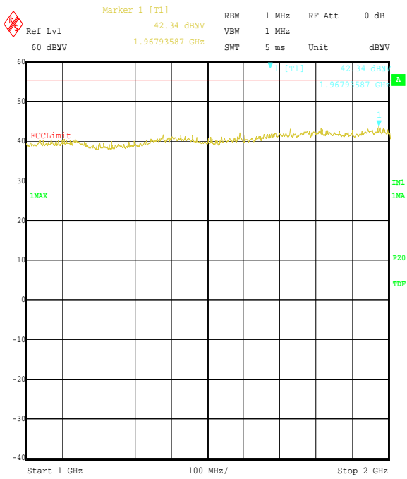
Title: Ezurio Test No 48271JD02 FCC Part 15.247 Comment A: Radiated Emissions Scans Top channel. BPSK OFDM Date: 6.SEP.2006 16:29:36
