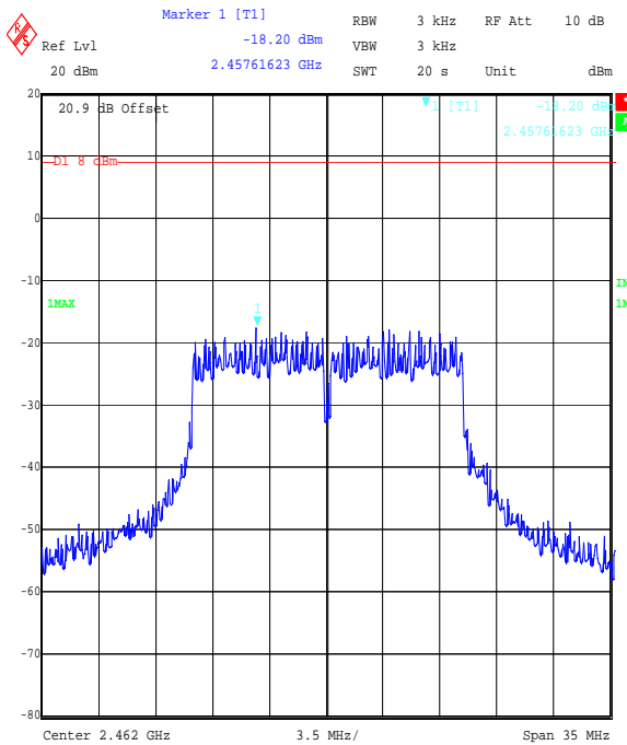
Title: EZURIO 2.4 GHz WLAN Module, FCC Part 15.247 Spectral Density Comment A: 48271JD05 Top Channel OFDM 64QAM Date: 8.SEP.2006 16:05:01
