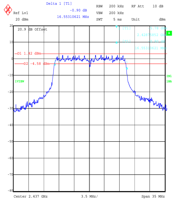
Title: Ezurio 2.4 GHz WLAN module. FCC P15.247 6 dB Bandwidth Comment A: 48271JD05 Middle Channel, BPSK OFDM. Date: 5.SEP.2006 16:23:31
