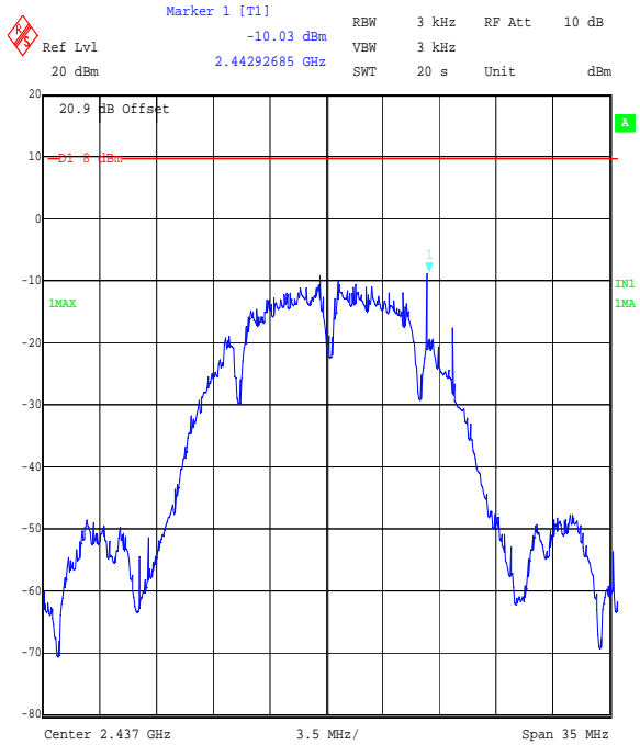
Title: Ezurio 2.4 GHz WLAN module, FCC P15.247 Spectral Density Comment A: 48271JD05 Middle Channel, BPSK DSSS. Date: 5.SEP.2006 14:26:22
