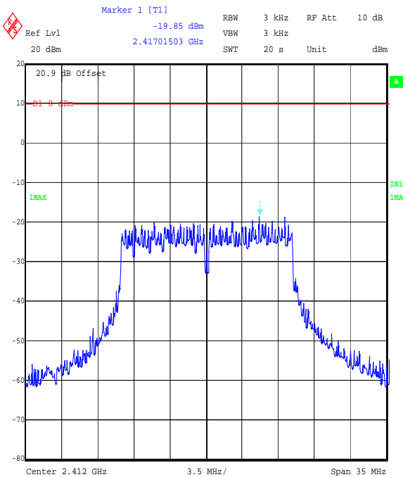
Title: Ezurio 2.4 GHz WLAN module, FCC P15.247 Spectral Density Comment A: 48271JD05 Bottom Channel, 64QAM OFDM. Date: 5.SEP.2006 14:19:38
