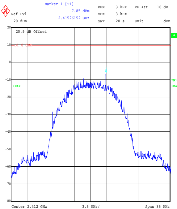
Title: Ezurio 2.4 GHz WLAN module, FCC P15.247 Spectral Density Comment A: 48271JD05 Bottom Channel, QPSK DSSS. Date: 5.SEP.2006 14:13:16
