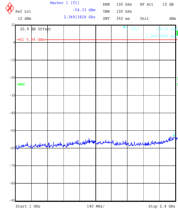
Title: EZURIO 2.4 GHz WLAN Module, FCC Part 15.247 Cond. Emissions Comment A: 48271JD05 Top Channel OFDM BPSK Date: 8.SEP.2006 16:51:05
