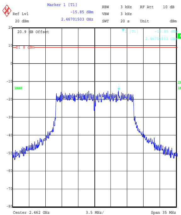
Title: EZURIO 2.4 GHz WLAN Module, FCC Part 15.247 Spectral Density Comment A: 48271JD05 Top Channel OFDM BPSK Date: 8.SEP.2006 16:12:03
