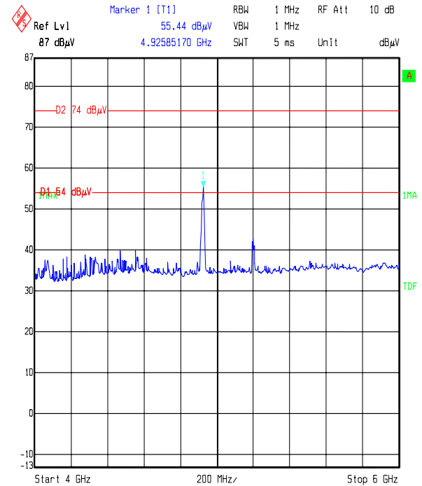
Comment A: Radiated emissions DSSS, CCK 4-6GHz Date: 12.OCT.2006 16:40:40
