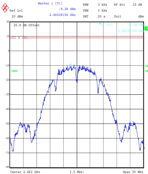
Title: EZURIO 2.4 GHz WLAN Module, FCC Part 15.247 Spectral Density Comment A: 48271JD05 Top Channel DSSS BPSK Date: 8.SEP.2006 16:16:04
