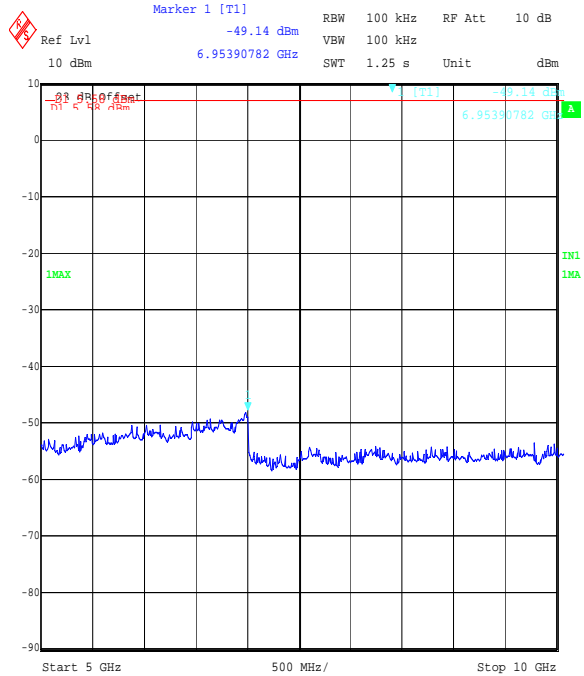
Title: EZURIO 2.4 GHz WLAN Module, FCC Part 15.247 Cond. Emissions Comment A: 48271JD05 Top Channel DSSS BPSK Date: 8.SEP.2006 17:03:05
