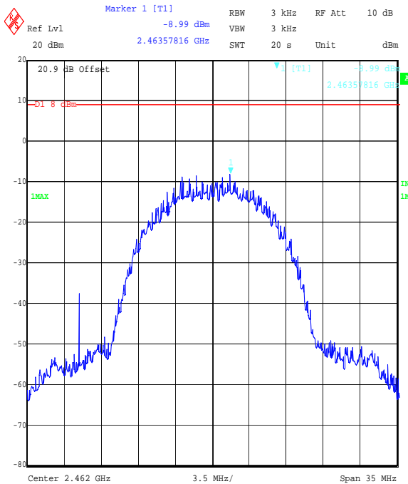
Title: EZURIO 2.4 GHz WLAN Module, FCC Part 15.247 Spectral Density Comment A: 48271JD05 Top Channel DSSS QPSK Date: 8.SEP.2006 16:14:43
