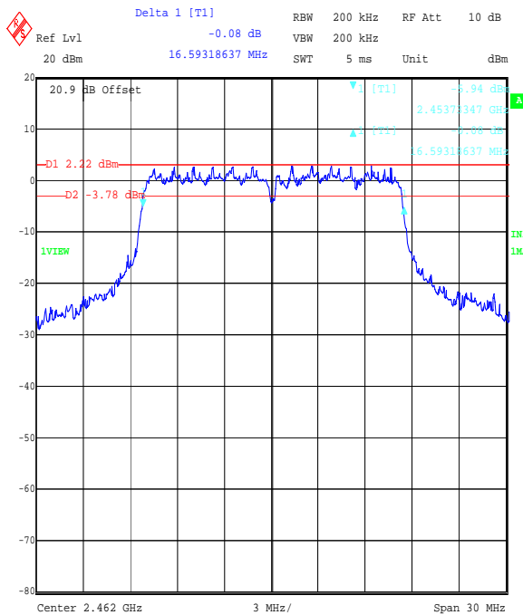
Title: EZURIO 2.4 GHz WLAN Module. FCC Part 15.247 6 dB Bandwidth Comment A: 48271JD05 Top Channel OFDM BPSK Date: 8.SEP.2006 15:55:27
