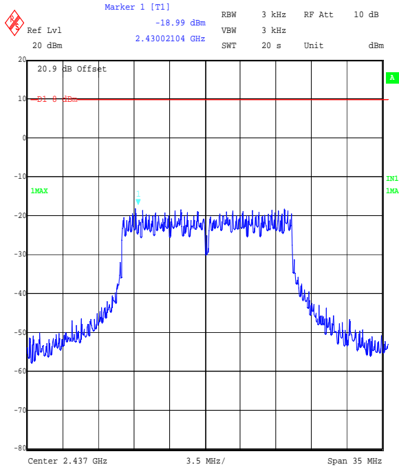
Title: Ezurio 2.4 GHz WLAN module, FCC P15.247 Spectral Density Comment A: 48271JD05 Middle Channel, 16QAM OFDM. Date: 5.SEP.2006 14:24:23
