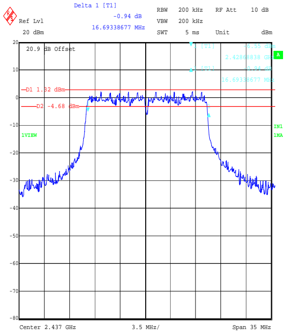
Title: Ezurio 2.4 GHz WLAN module, FCC P15.247 6 dB Bandwidth Comment A: 48271JD05 Middle Channel, 16QAM OFDM. Date: 5.SEP.2006 16:27:39
