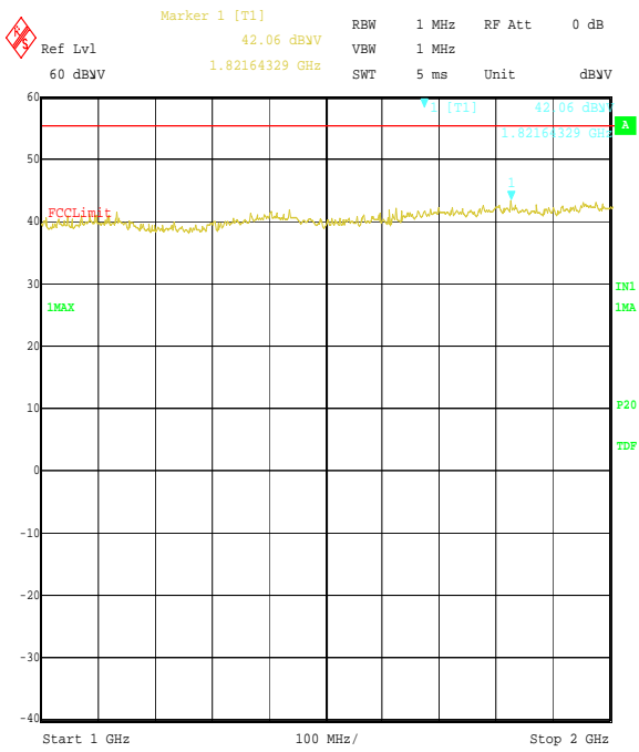
Title: Ezurio Test No 48271JD02 FCC Part 15.247 Comment A: Radiated Emissions Scans Top channel. CCK DSSS Date: 6.SEP.2006 16:30:55
