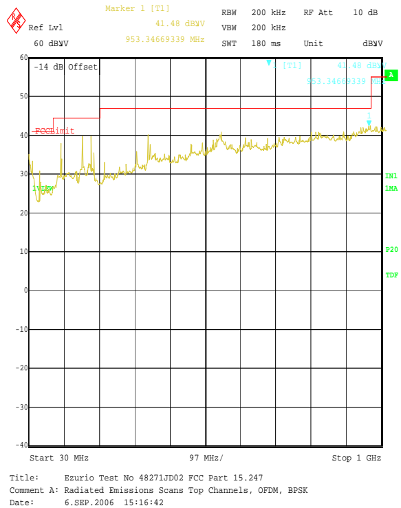
Pre-scan with 3 dBi antenna
