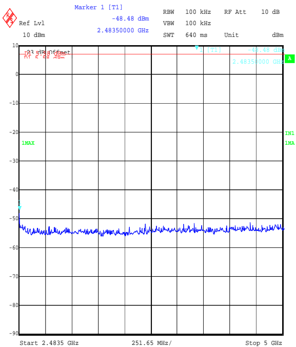
Title: EZURIO 2.4 GHz WLAN Module, FCC Part 15.247 Cond. Emissions Comment A: 48271JD05 Top Channel DSSS BPSK Date: 8.SEP.2006 17:03:23
