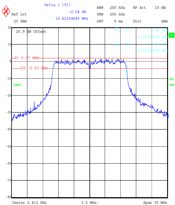
Title: Ezurio 2.4 GHz WLAN module. FCC P15.247 6 dB Bandwidth Comment A: 48271JD05 Bottom Channel, BPSK OFDM. Date: 5.SEP.2006 16:37:10
