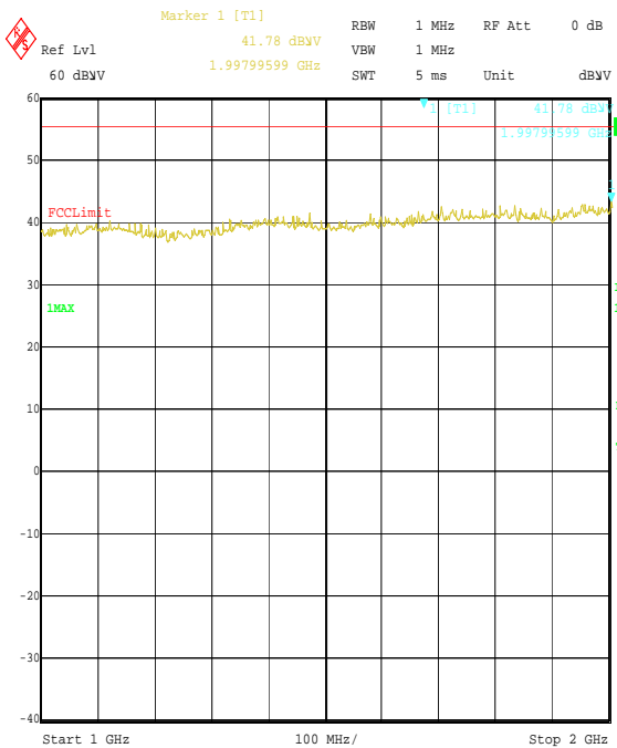
Title: Ezurio Test No 48271JD02 FCC Part 15.247 Comment A: Radiated Emissions Scans Rx Mode Date: 6.SEP.2006 16:15:16
