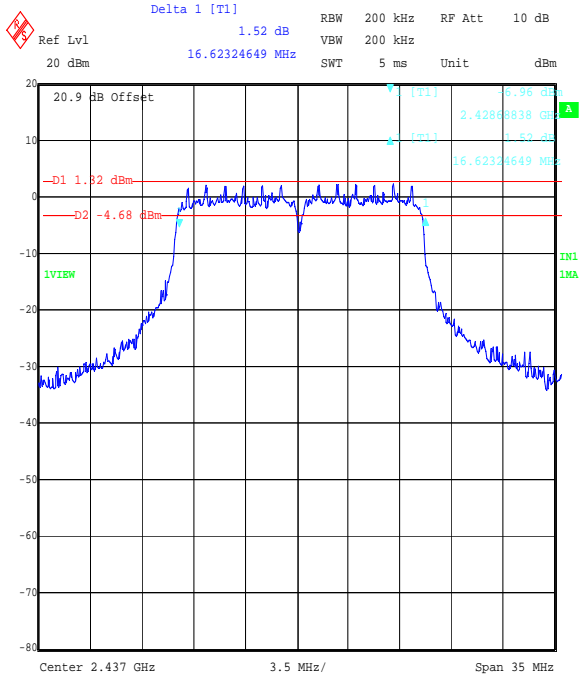
Title: Ezurio 2.4 GHz WLAN module. FCC P15.247 6 dB Bandwidth Comment A: 48271JD05 Middle Channel, QPSK OFDM. Date: 5.SEP.2006 16:24:59
