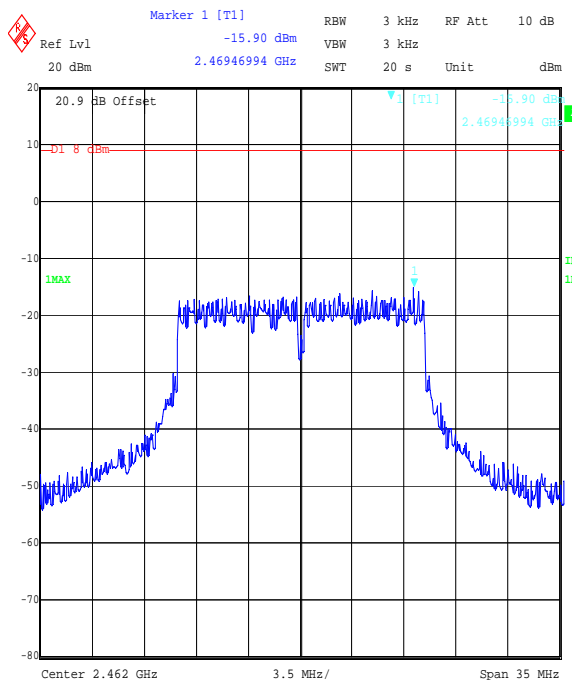
Title: EZURIO 2.4 GHz WLAN Module, FCC Part 15.247 Spectral Density Comment A: 48271JD05 Top Channel OFDM QPSK Date: 8.SEP.2006 16:07:17
