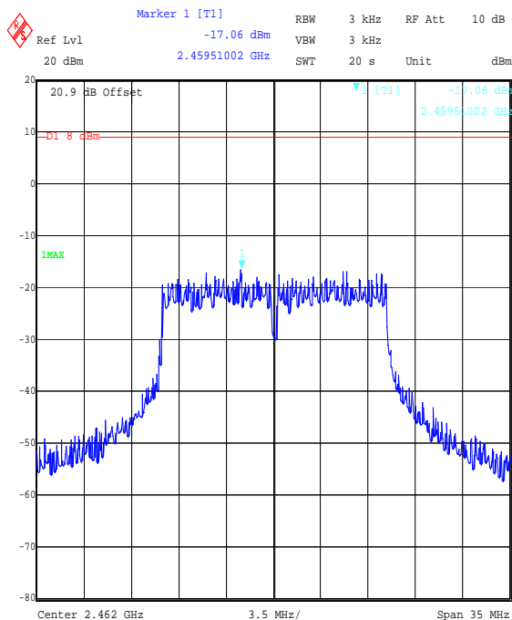
Title: EZURIO 2.4 GHz WLAN Module, FCC Part 15.247 Spectral Density Comment A: 48271JD05 Top Channel OFDM 16QAM Date: 8.SEP.2006 16:06:18
