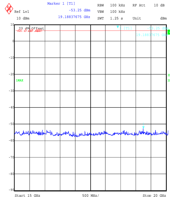
Title: EZURIO 2.4 GHz WLAN Module, FCC Part 15.247 Cond. Emissions Comment A: 48271JD05 Top Channel DSSS BPSK Date: 8.SEP.2006 17:02:20
