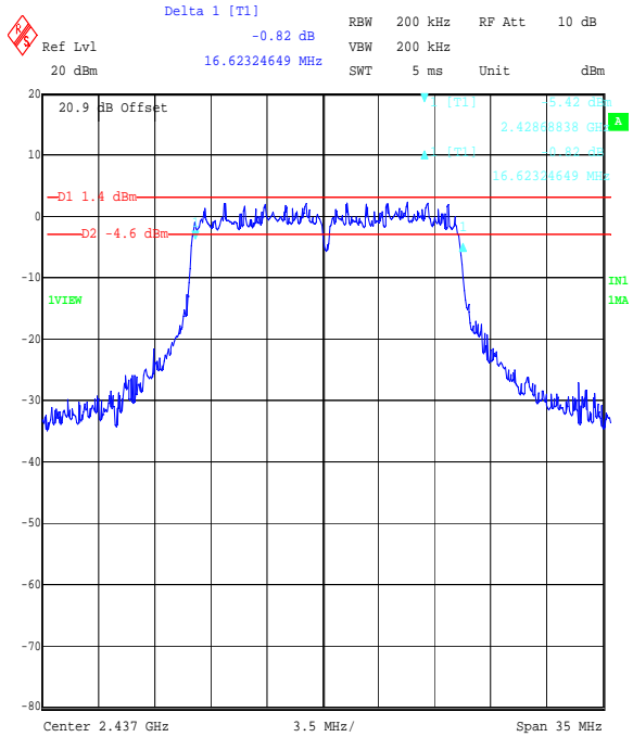
Title: Ezurio 2.4 GHz WLAN module, FCC P15.247 6 dB Bandwidth Comment A: 48271JD05 Middle Channel, 64QAM OFDM. Date: 5.SEP.2006 16:28:44
