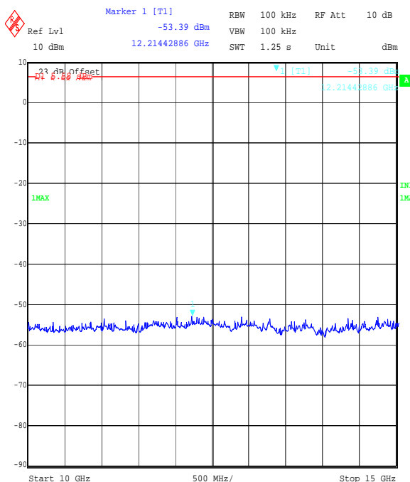
Title: EZURIO 2.4 GHz WLAN Module, FCC Part 15.247 Cond. Emissions Comment A: 48271JD05 Top Channel DSSS BPSK Date: 8.SEP.2006 17:02:45
