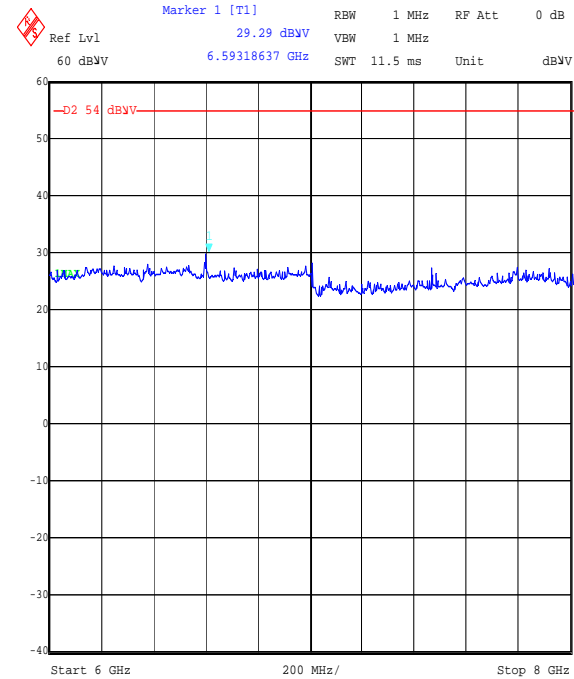
Title: Ezurio 2.4GHz WLAN FCC P15.247 Radiated Emissions Comment A: 48271JD05 RX mode Date: 7.SEP.2006 14:44:44
