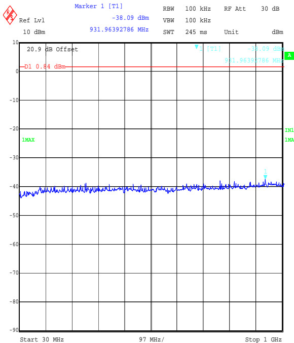
Title: EZURIO 2.4 GHz WLAN Module, FCC Part 15.247 Cond. Emissions Comment A: 48271JD05 Top Channel OFDM BPSK Date: 8.SEP.2006 16:50:41
