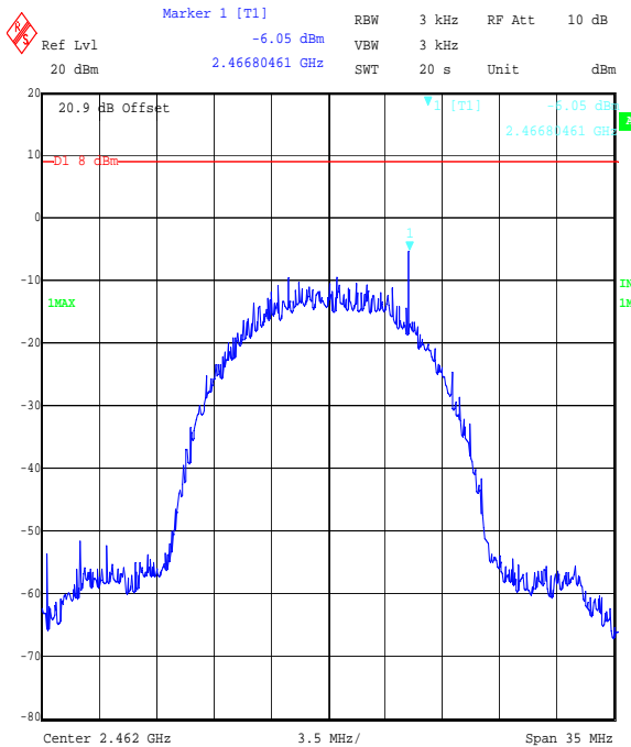
Title: EZURIO 2.4 GHz WLAN Module, FCC Part 15.247 Spectral Density Comment A: 48271JD05 Top Channel DSSS CCK Date: 8.SEP.2006 16:13:21
