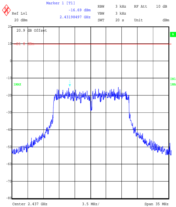
Title: Ezurio 2.4 GHz WLAN module, FCC P15.247 Spectral Density Comment A: 48271JD05 Middle Channel, QPSK OFDM. Date: 5.SEP.2006 14:23:46
