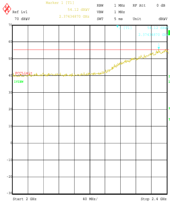
Title: Ezurio Test No 48271JD02 FCC Part 15.247 Comment A: Radiated Emissions Scans Top channel. CCK DSSS Date: 6.SEP.2006 17:31:15
