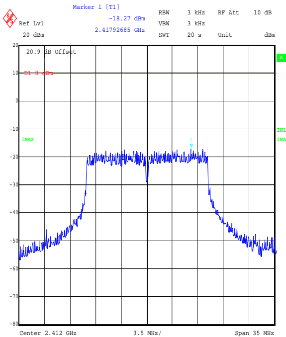
Title: Ezurio 2.4 GHz WLAN module, FCC P15.247 Spectral Density Comment A: 48271JD05 Bottom Channel, BPSK OFDM. Date: 5.SEP.2006 14:21:55
