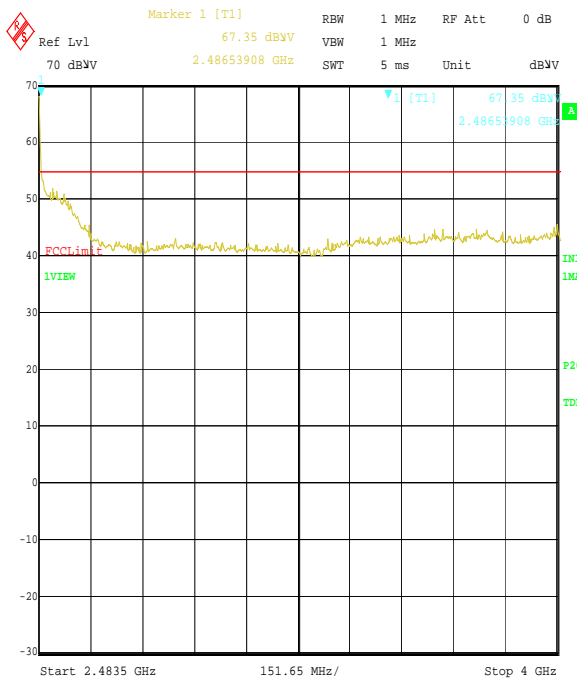
Title: Ezurio Test No 48271JD02 FCC Part 15.247 Comment A: Radiated Emissions Scans Top channel. CCK DSSS Date: 6.SEP.2006 17:27:49
