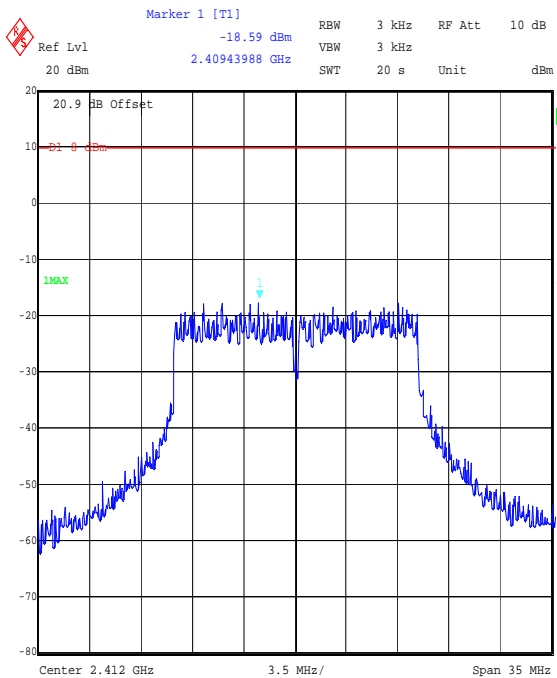
Title: Ezurio 2.4 GHz WLAN module, FCC P15.247 Spectral Density Comment A: 48271JD05 Bottom Channel, 16QAM OFDM. Date: 5.SEP.2006 14:20:35
