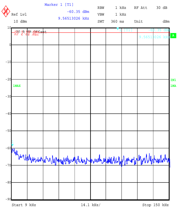
Title: EZURIO 2.4 GHz WLAN Module, FCC Part 15.247 Cond. Emissions Comment A: 48271JD05 Top Channel DSSS BPSK Date: 8.SEP.2006 17:04:38
