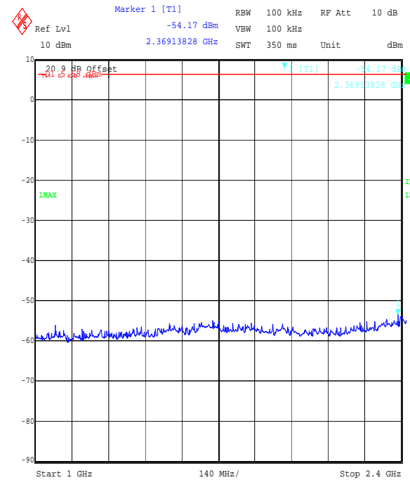
Title: EZURIO 2.4 GHz WLAN Module, FCC Part 15.247 Cond. Emissions Comment A: 48271JD05 Top Channel DSSS BPSK Date: 8.SEP.2006 17:03:43
