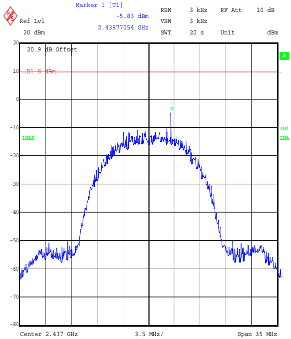
Title: Ezurio 2.4 GHz WLAN module, FCC P15.247 Spectral Density Comment A: 48271JD05 Middle Channel, CCK DSSS. Date: 5.SEP.2006 14:27:49
