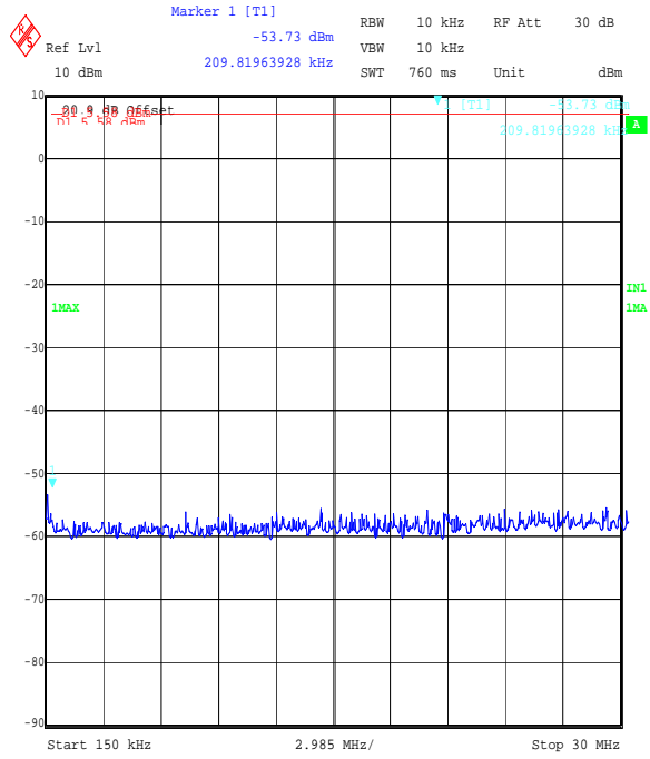
Title: EZURIO 2.4 GHz WLAN Module, FCC Part 15.247 Cond. Emissions Comment A: 48271JD05 Top Channel DSSS BPSK Date: 8.SEP.2006 17:04:20
