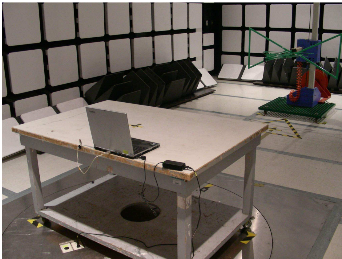
x-axis
