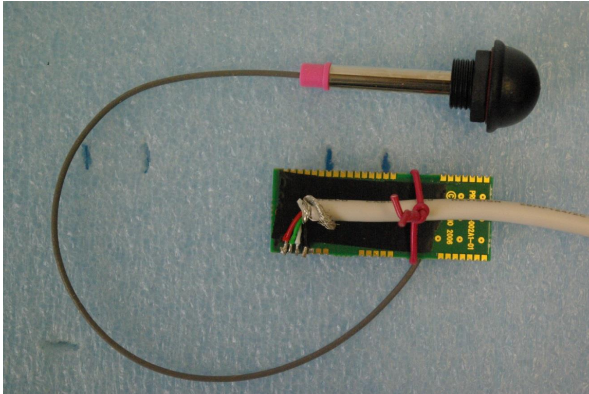
Photograph of EUT module and Antenna
