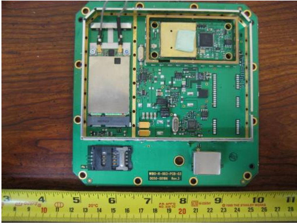
EUT – Main Board Component View
