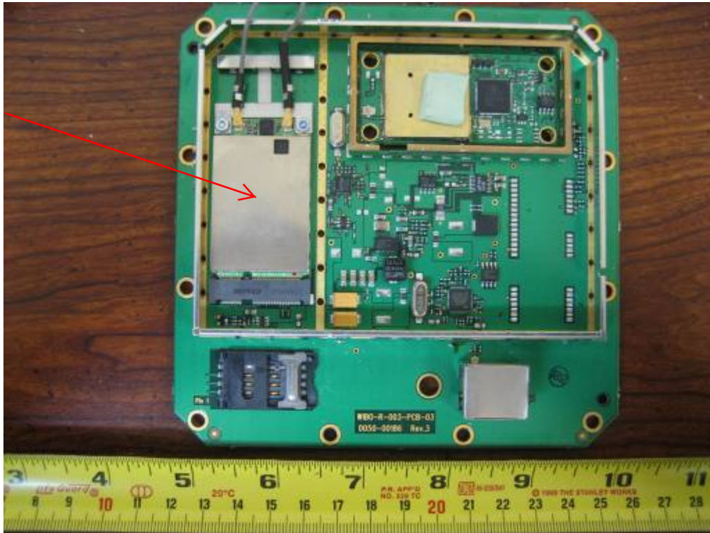
EUT – without RF Shielding view 2
