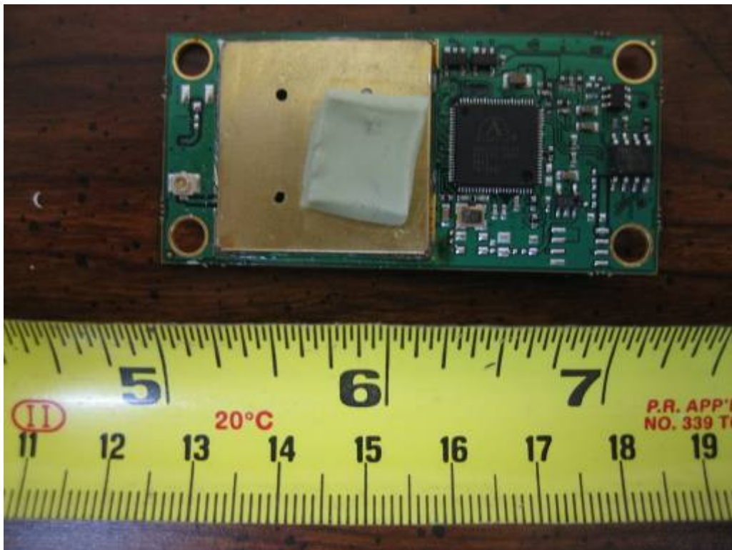
WLAN Board – Top View with RF Shielding
