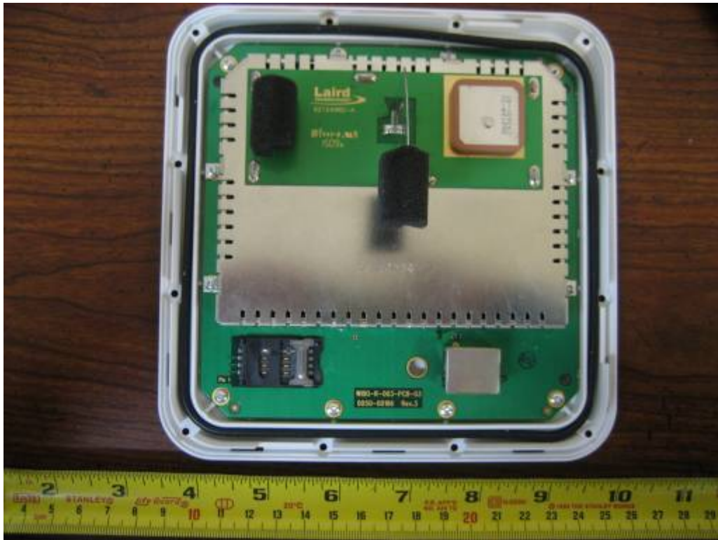
EUT – with RF Shielding
