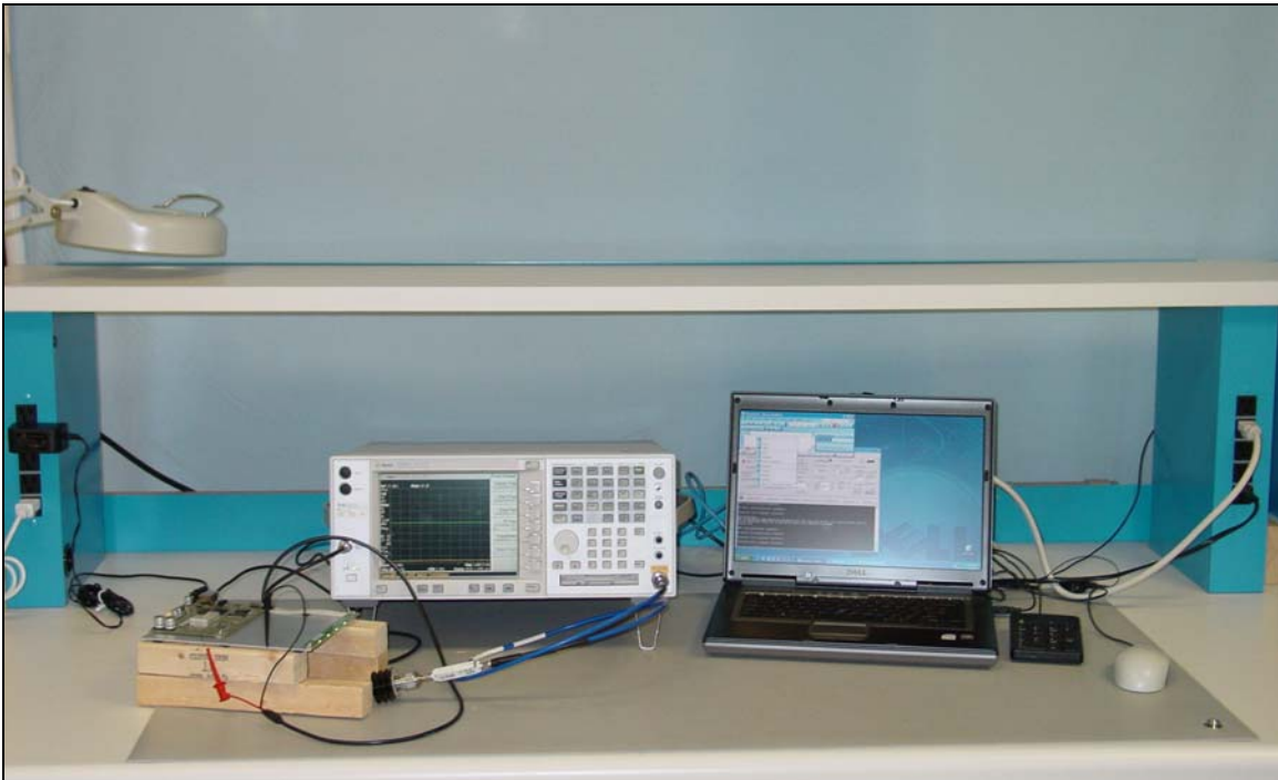
Transmit Harmonic Test Setup
