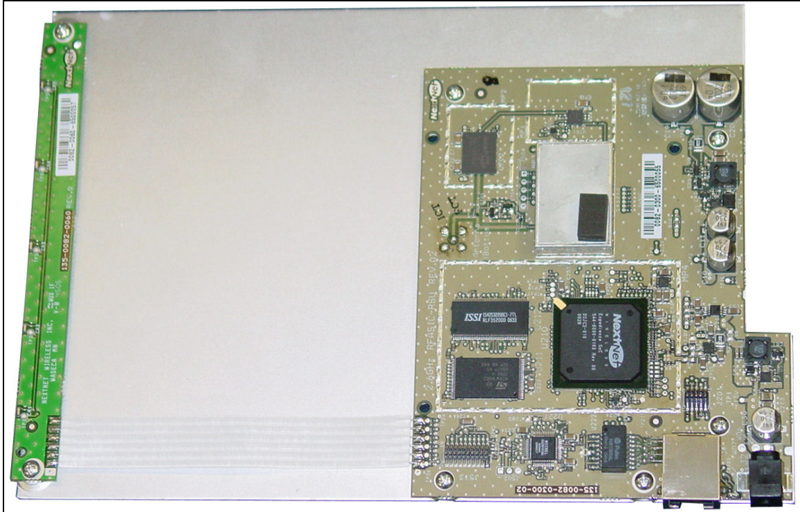
Main and LED Boards Component Side View (With Shield)
