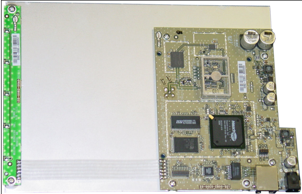
Main PC Board Component Side View (Without Shield)
