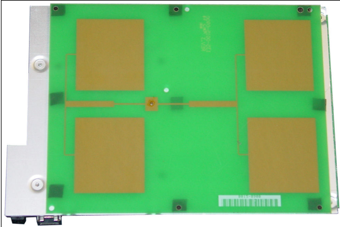
Vertical Antenna Board Bottom View
