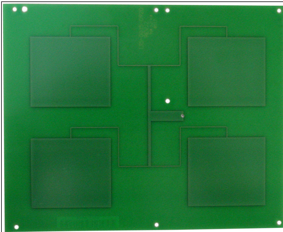
Horizontal Antenna Board Top View
