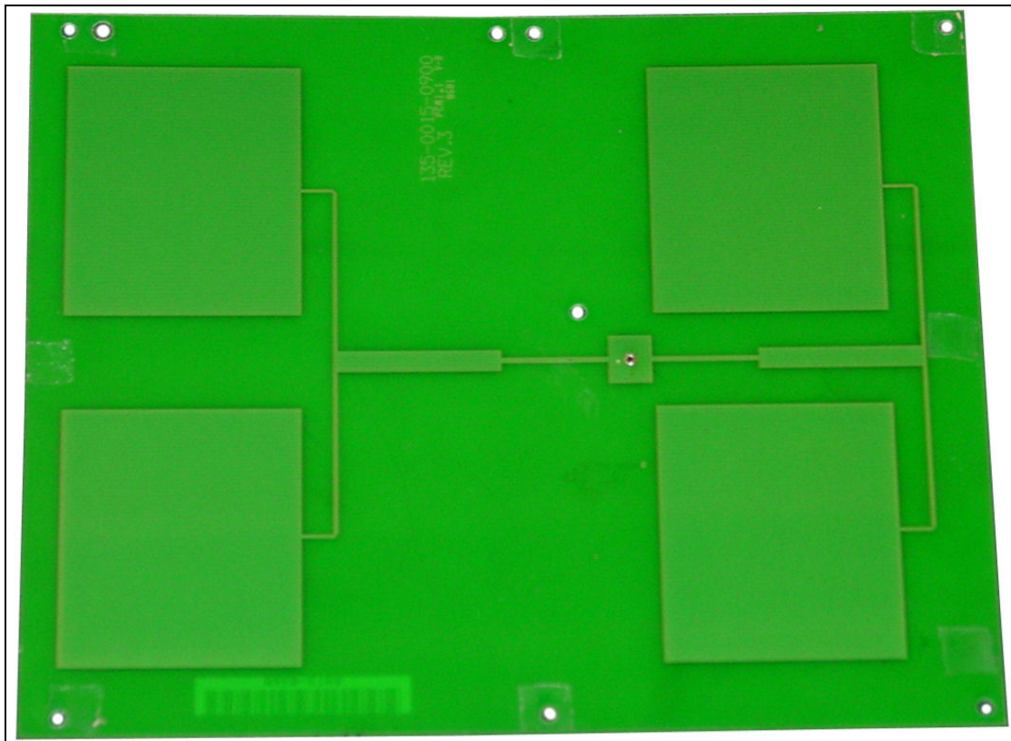
Vertical Antenna Board Top View
