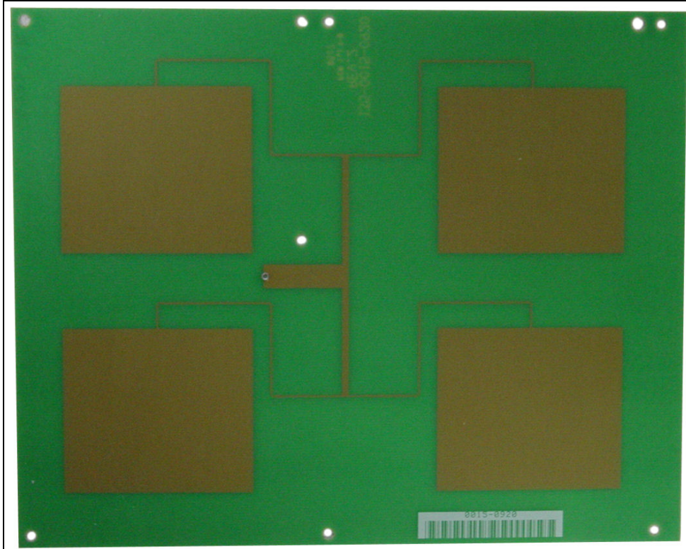
Horizontal Antenna Board Bottom View
