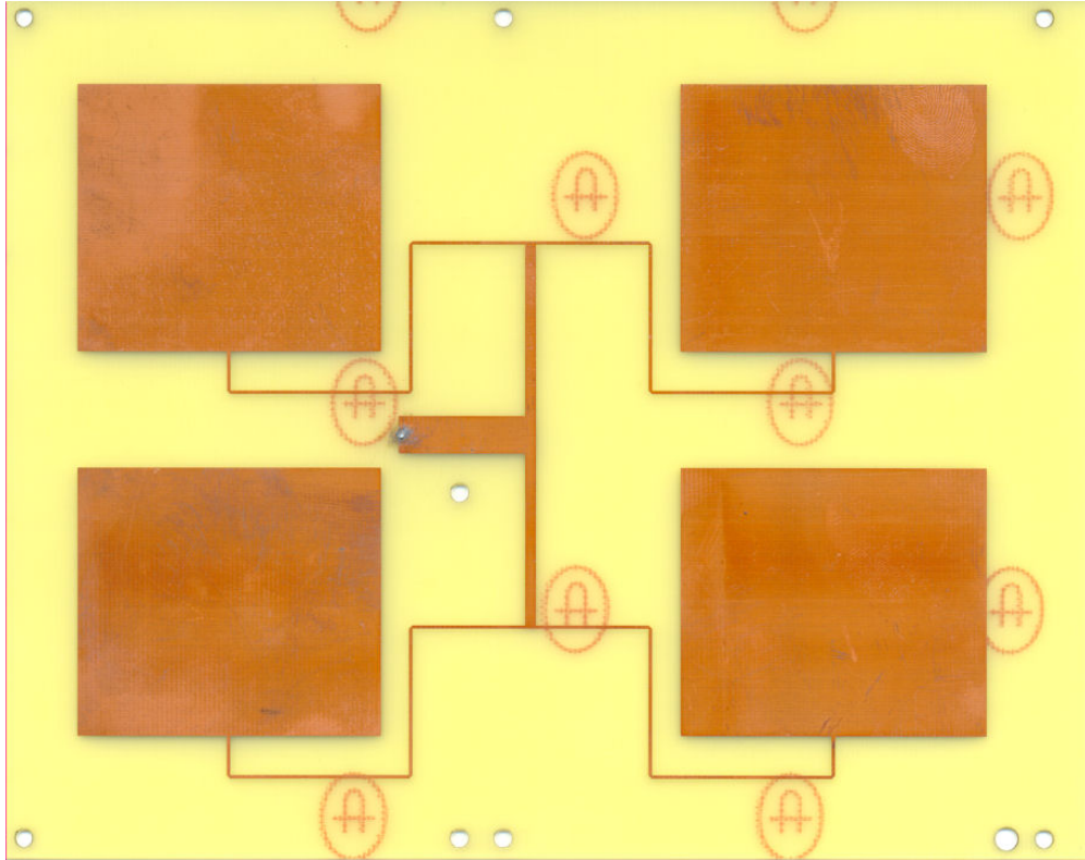
Horizontal Antenna Top Side View
