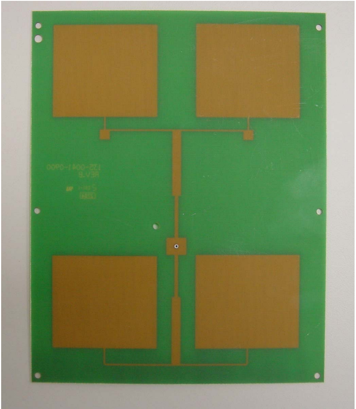
Vertically Polarized Antenna
