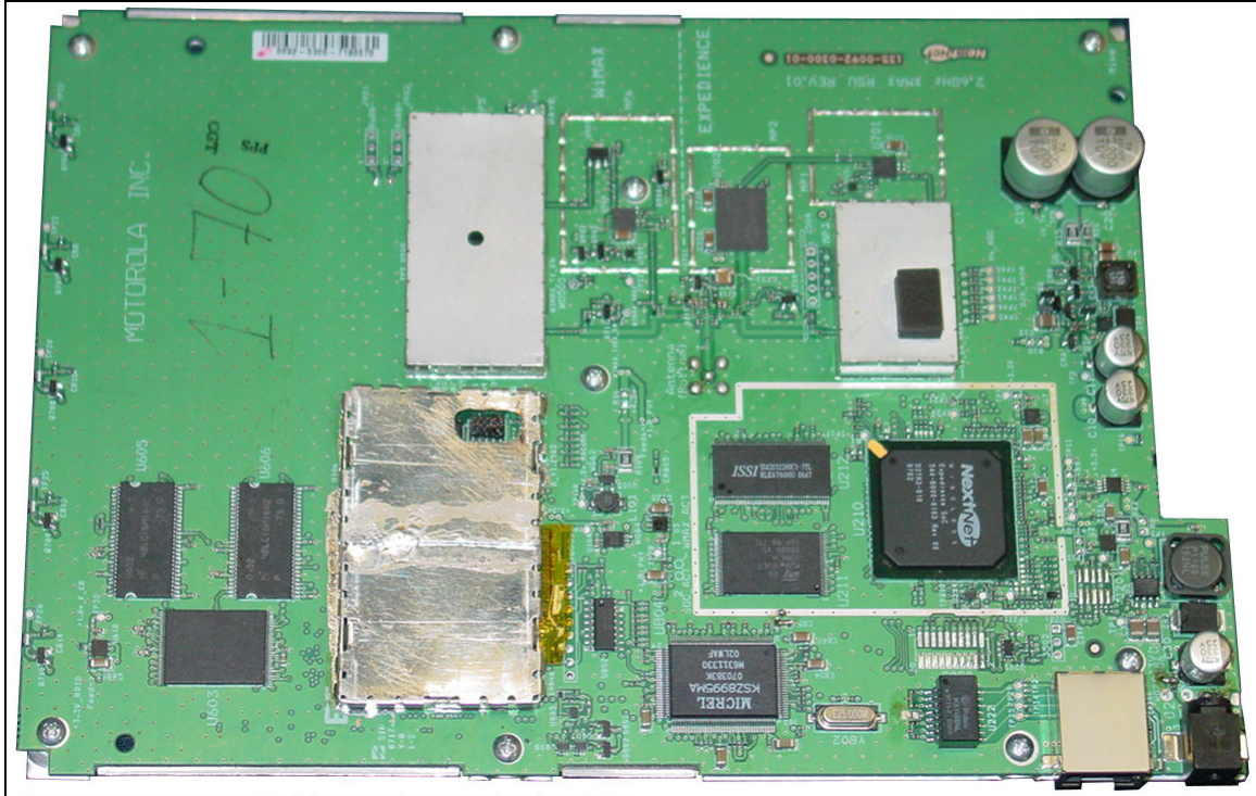
PC Board Component Side View (With Shields)
