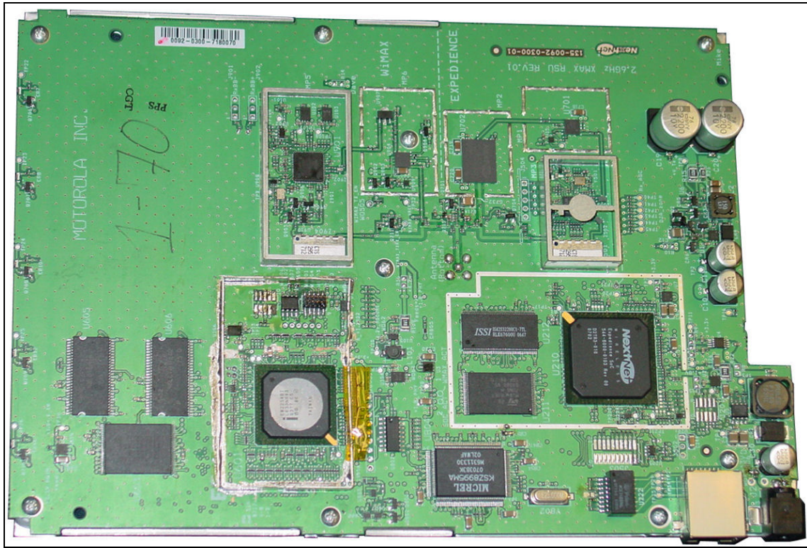
PC Board Component Side View (Without Shields)
