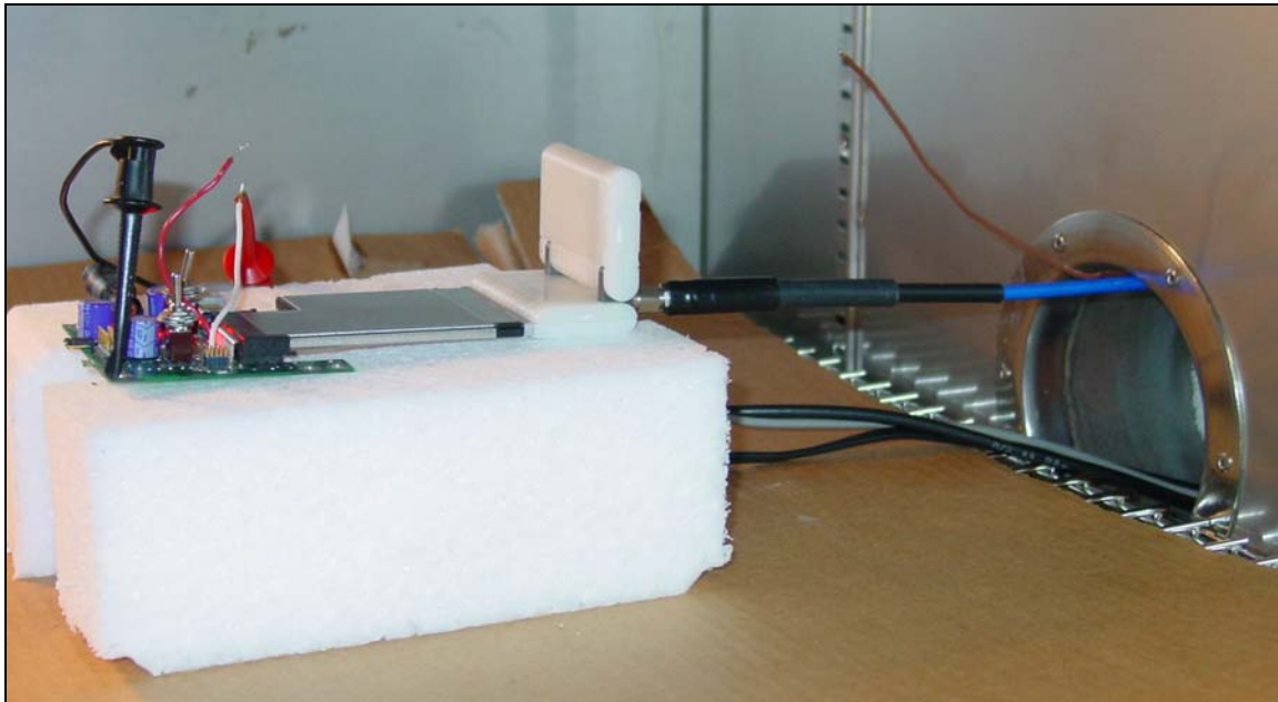
Frequency Stability Test Setup (Inside Chamber)
