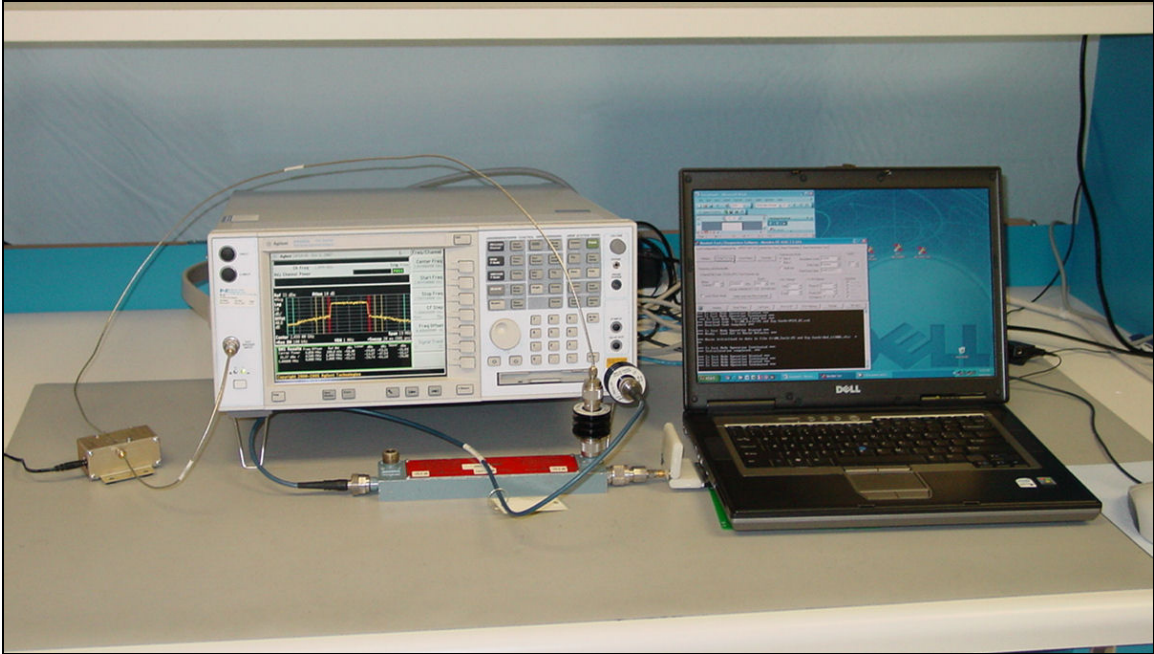
General Test Bench Setup
