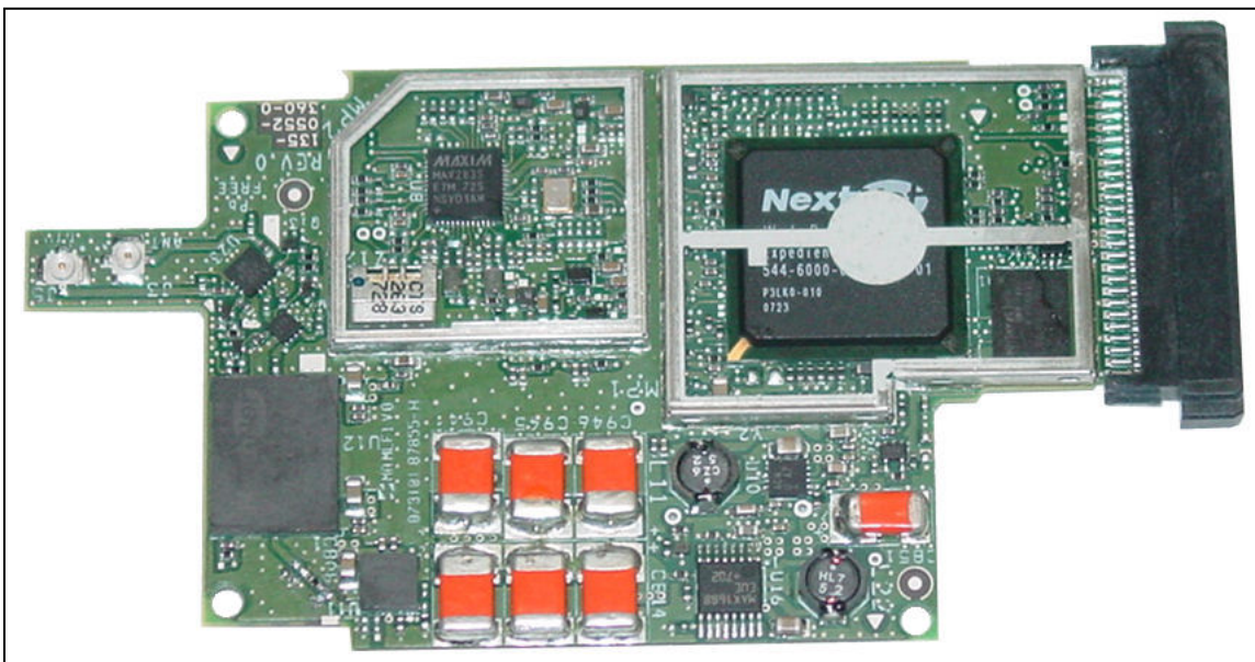
Main Board Top Side View (With Shield Covers Removed)
