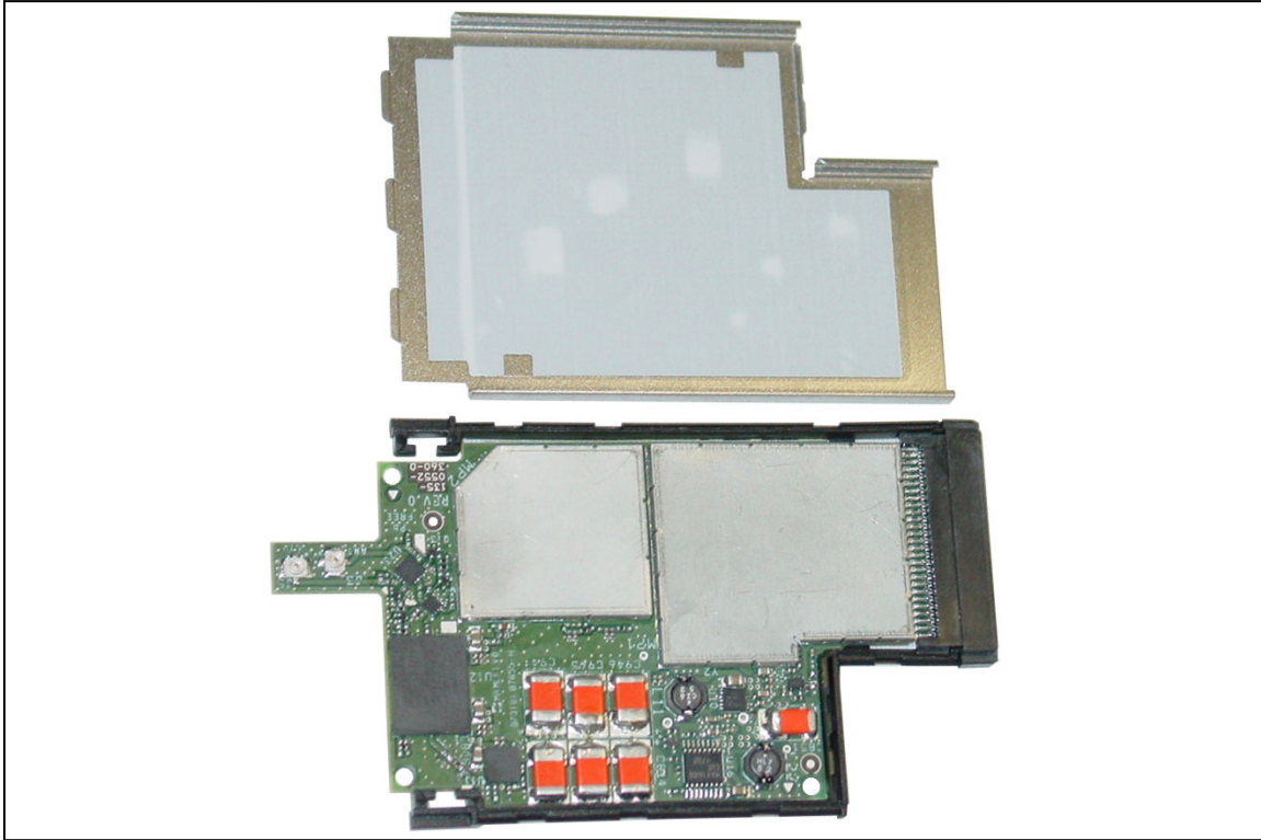
Top Cover
