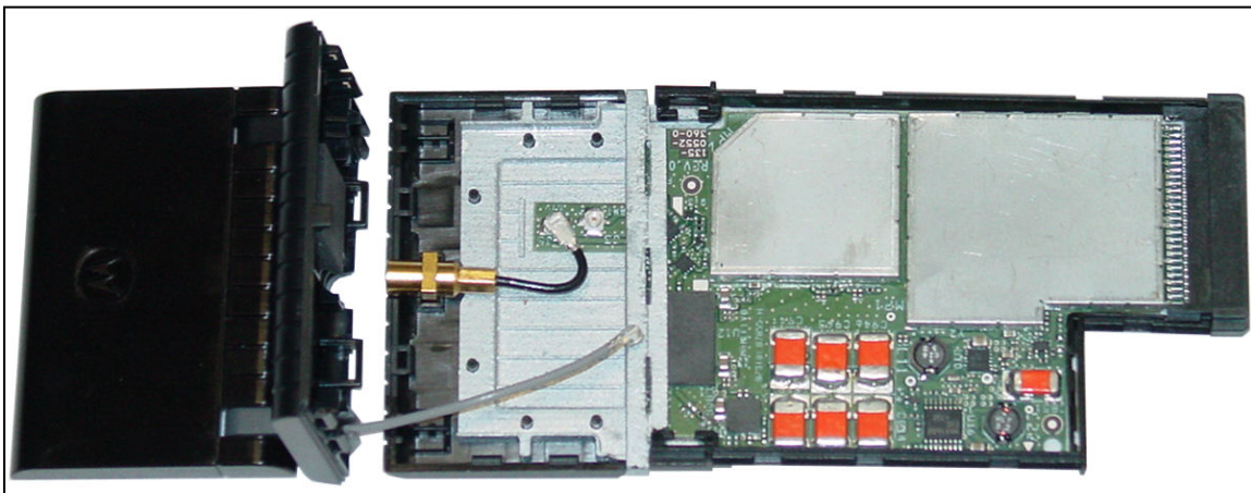
Antenna Base Internal View
