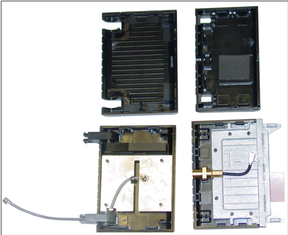
Antenna Assembly
