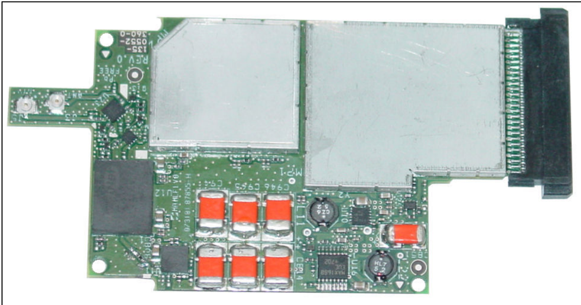
Main Board Top Side View (With Shield Covers Installed)
