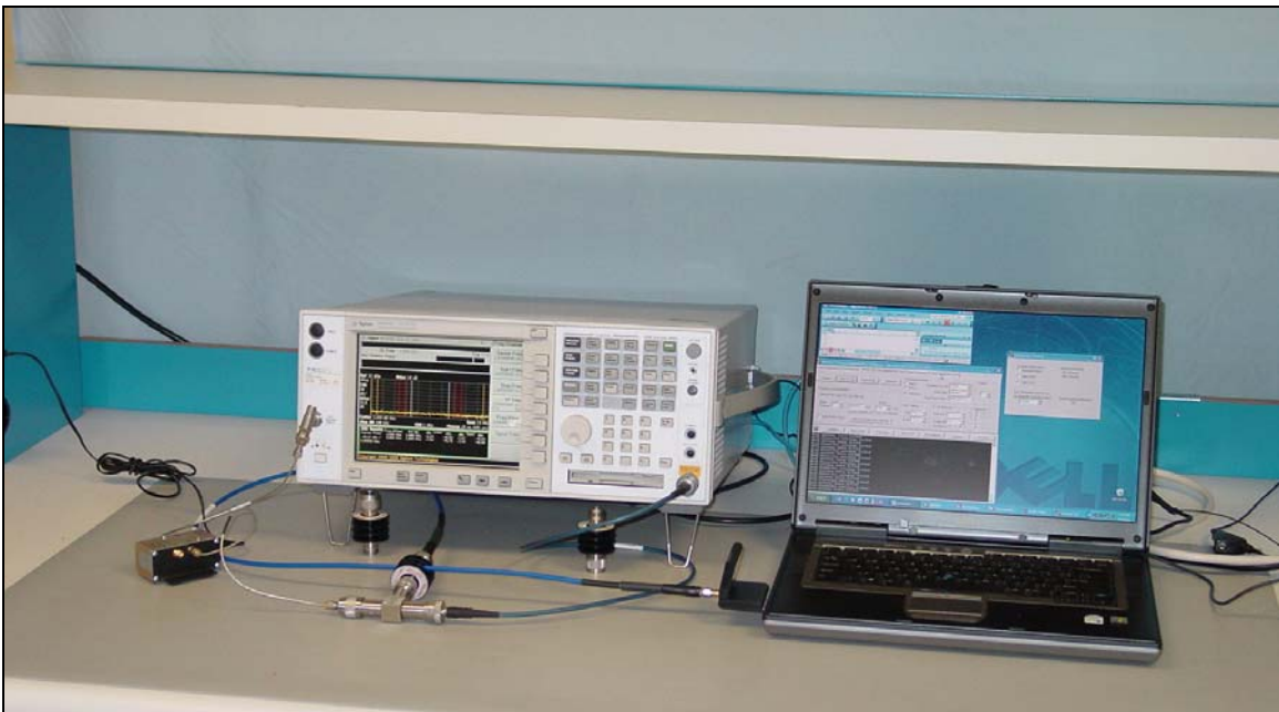
1 mW Power Output Test Setup
