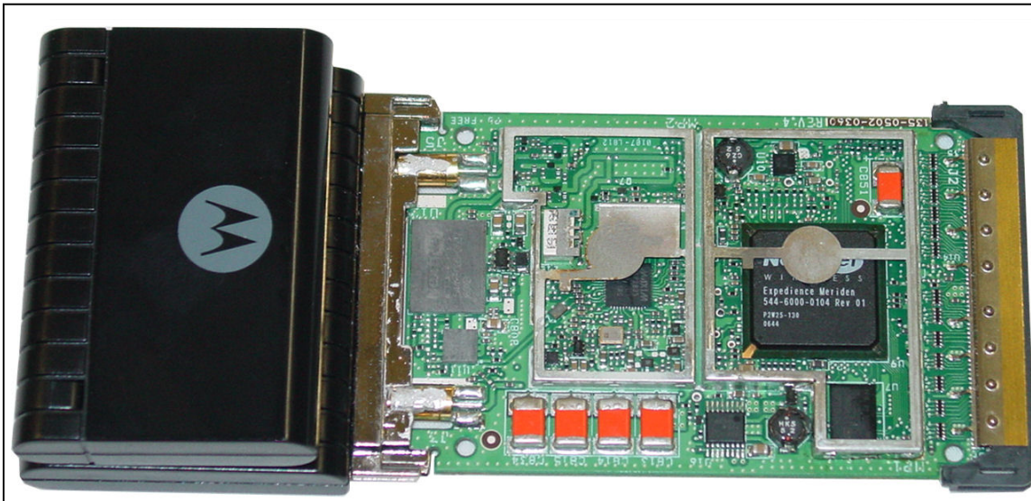
Main Board Top Side View (With Shield Covers Removed)
