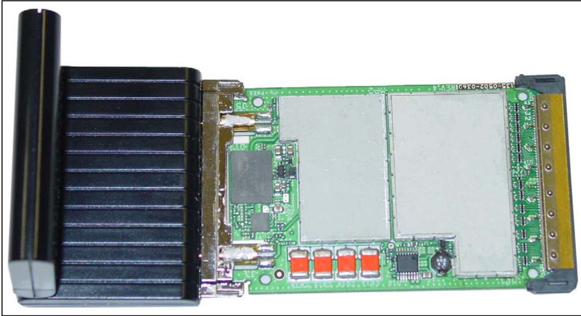
Main Board Top Side View (With Shield Covers Installed)
