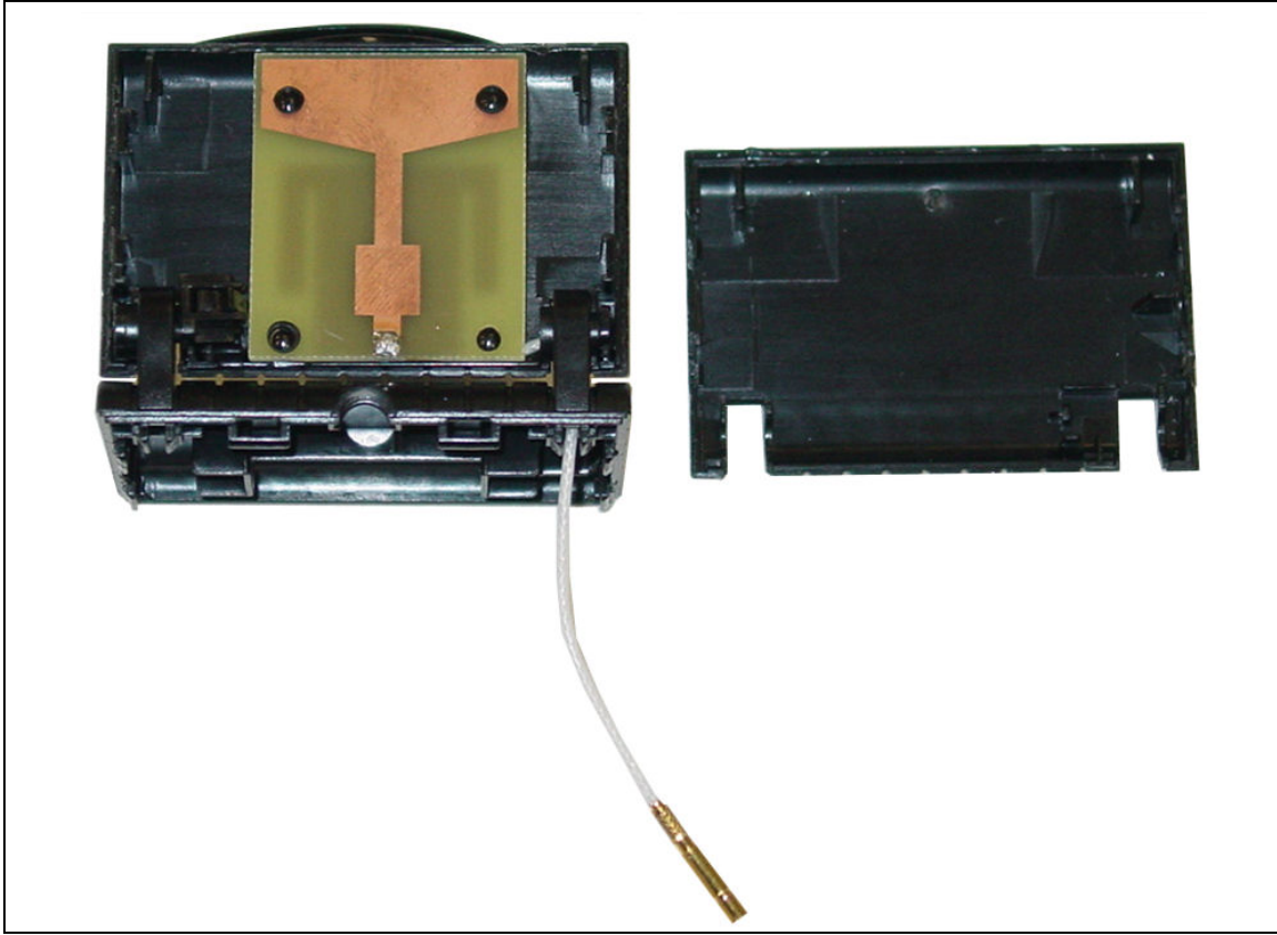
Antenna Board Back View
