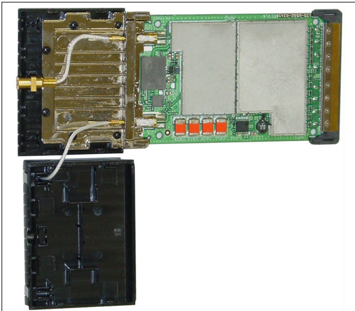
Antenna Base Internal View
