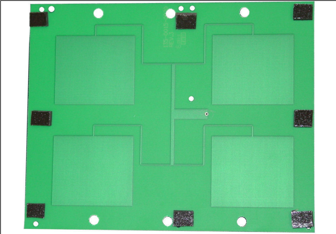
Antenna Board (Horiz Polarized) Inside View
