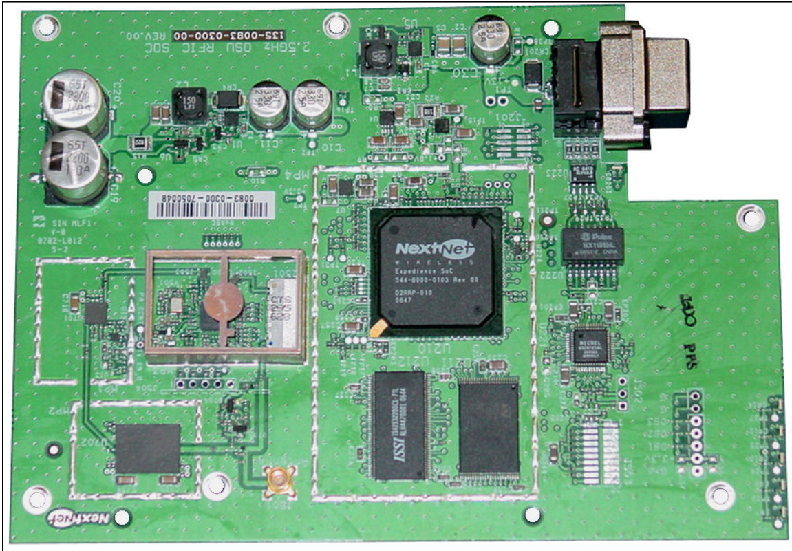
Main Board Top View (Shield Cover Removed)
