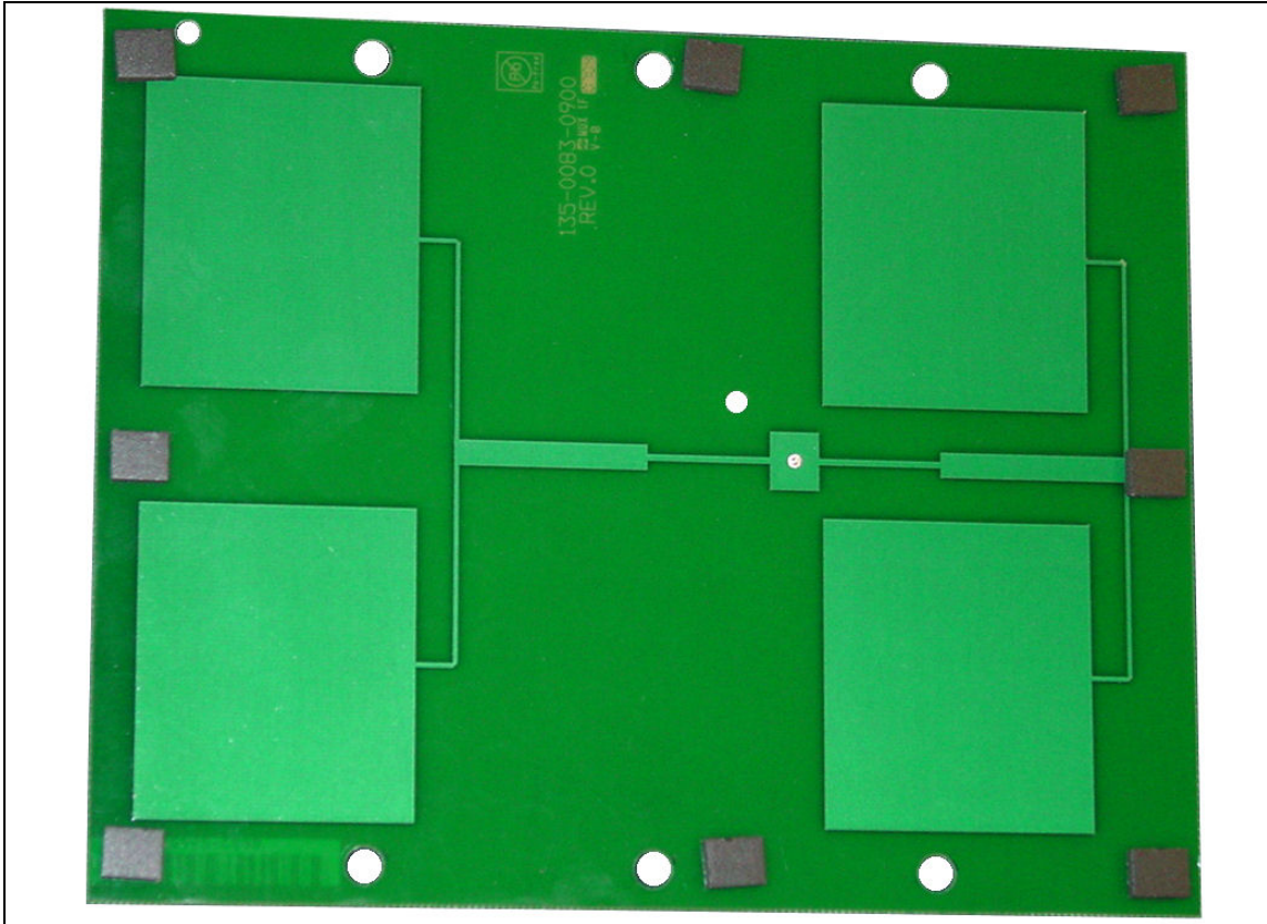
Antenna Board (Vert. Polarized) Inside View
