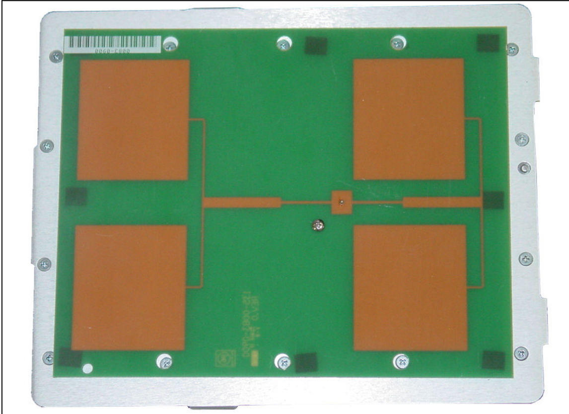
Antenna Board (Vert. Polarized) Outside View
