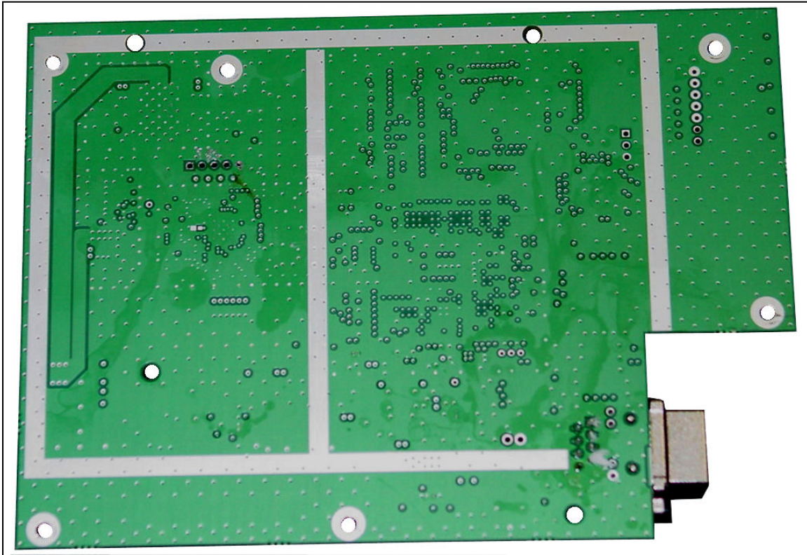
Main Board Bottom Side View
