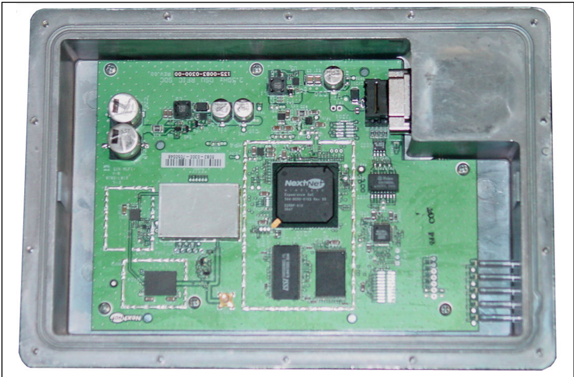
Main Board Installed in Chassis
