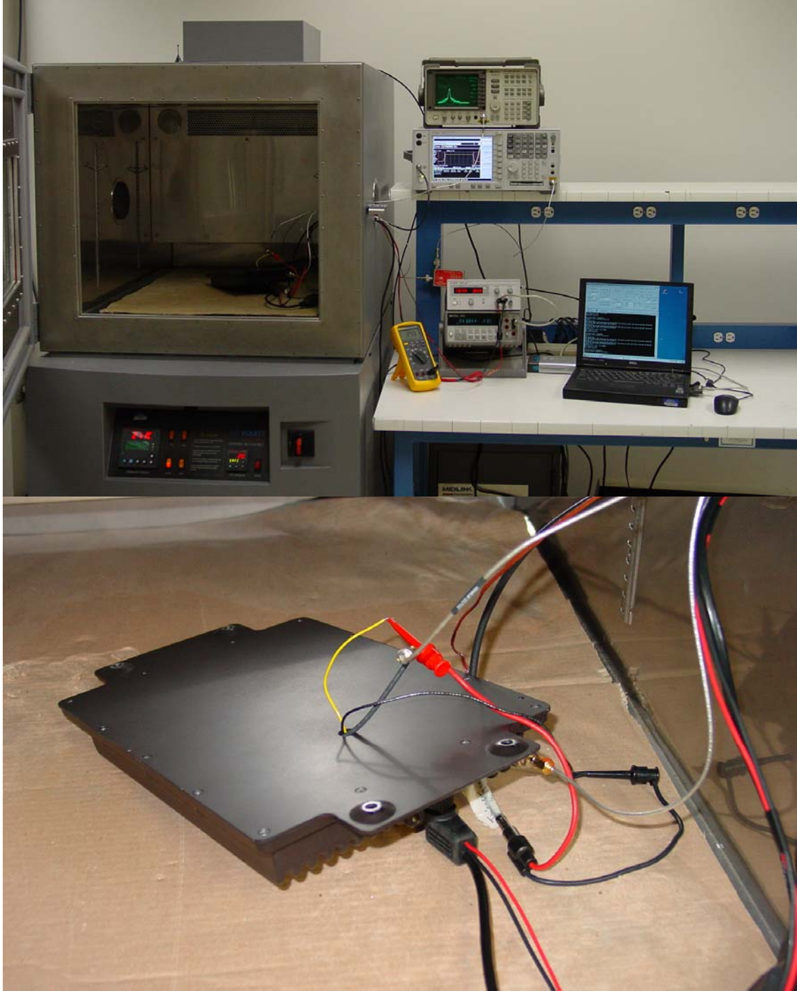
Frequency Stability
