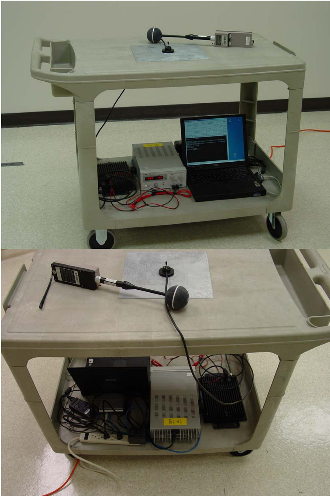
Radiation Hazard
