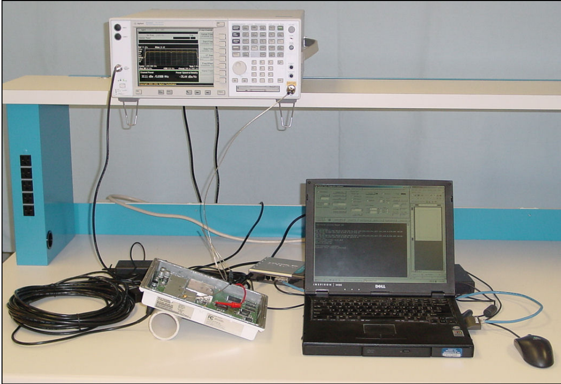
RF Power Out, Modulation Characteristics, Occupied Bandwidth, Spurious Emissions at Antenna Terminal
