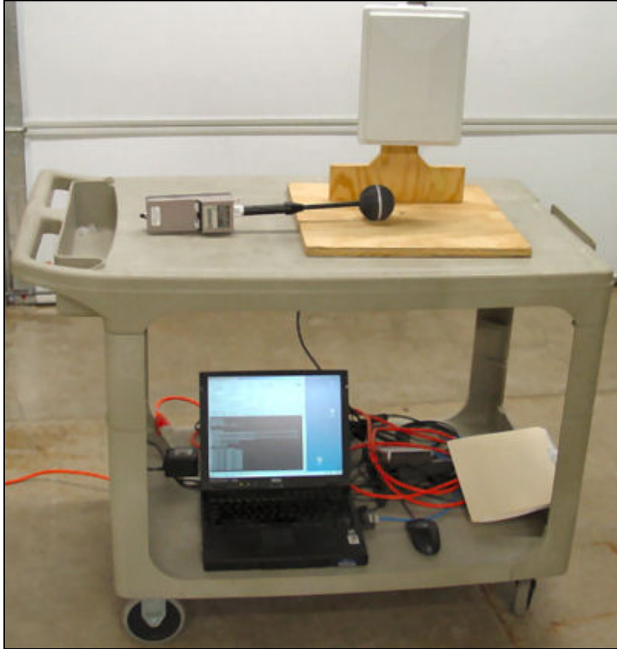
Radiation Hazard Test Setup
