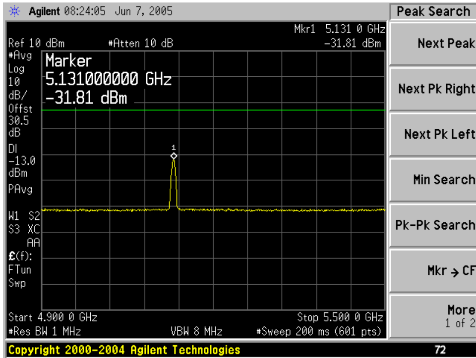
4.992 GHz – 5.38 GHz (2565.25 MHz / 5.5 MHz Channel / 2 nd Harmonic)
