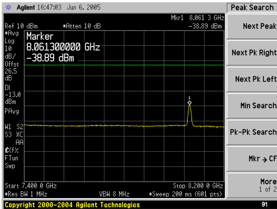
3 rd Harmonic of 2687.25 MHz
