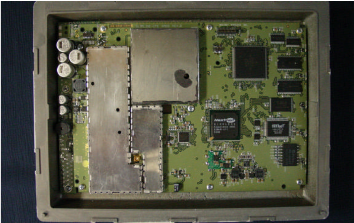
Main Board (component side / with shields)
