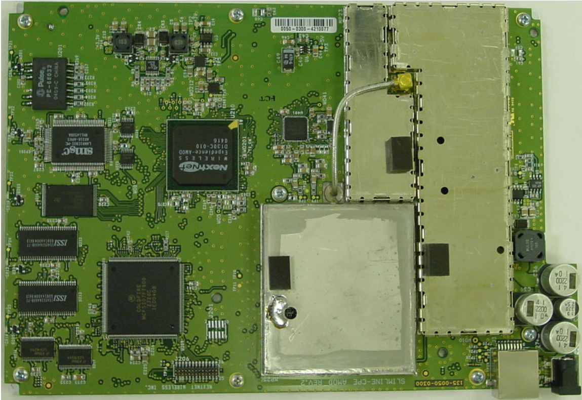
Main Board with Shields Installed, Top Side View
