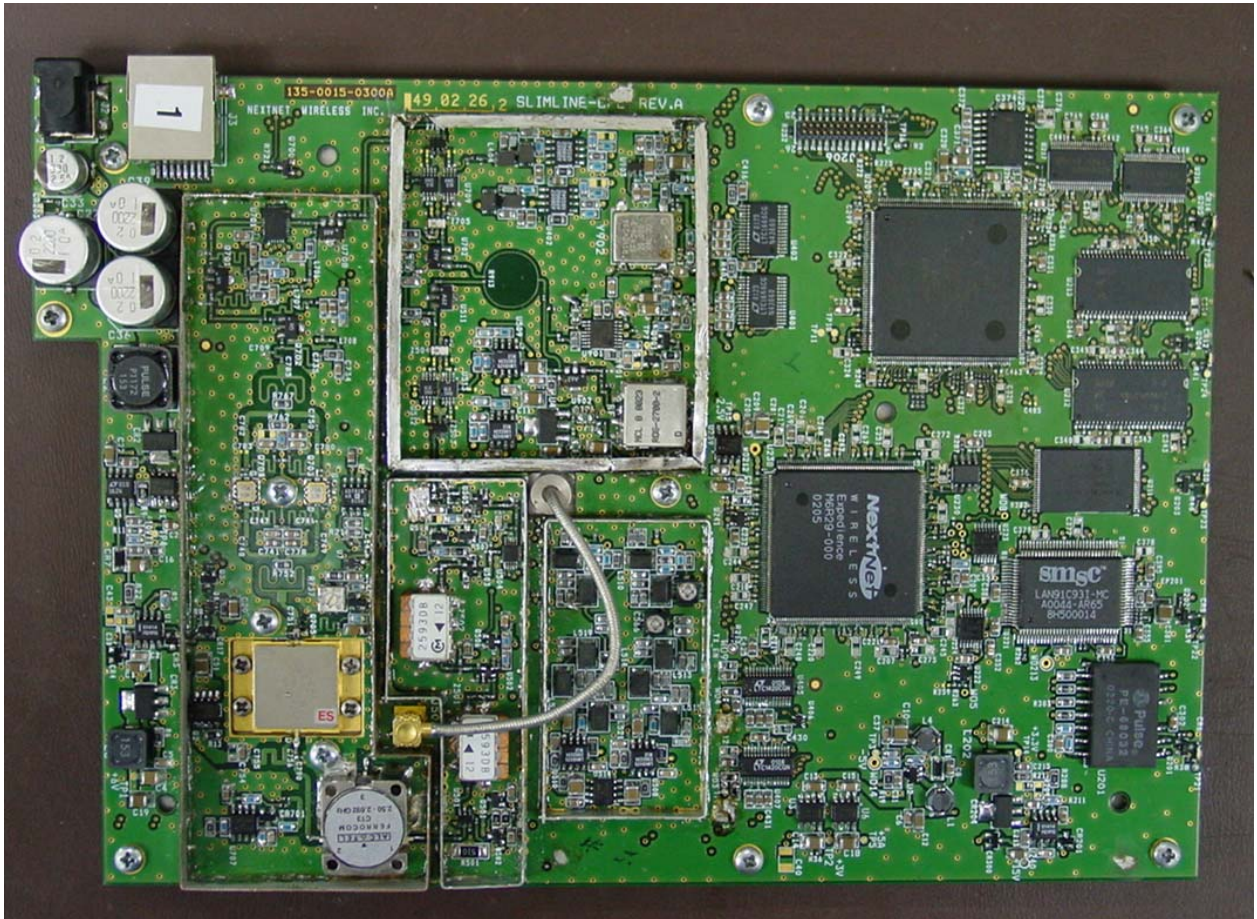
RF Board component side (no shields)
