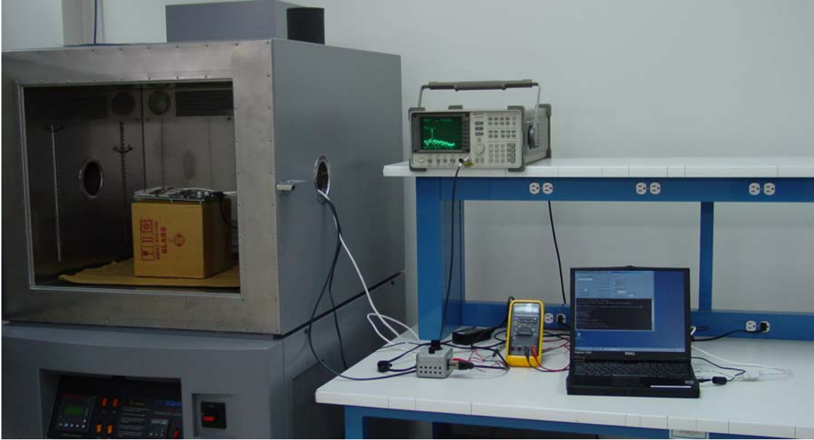
Frequency stability
