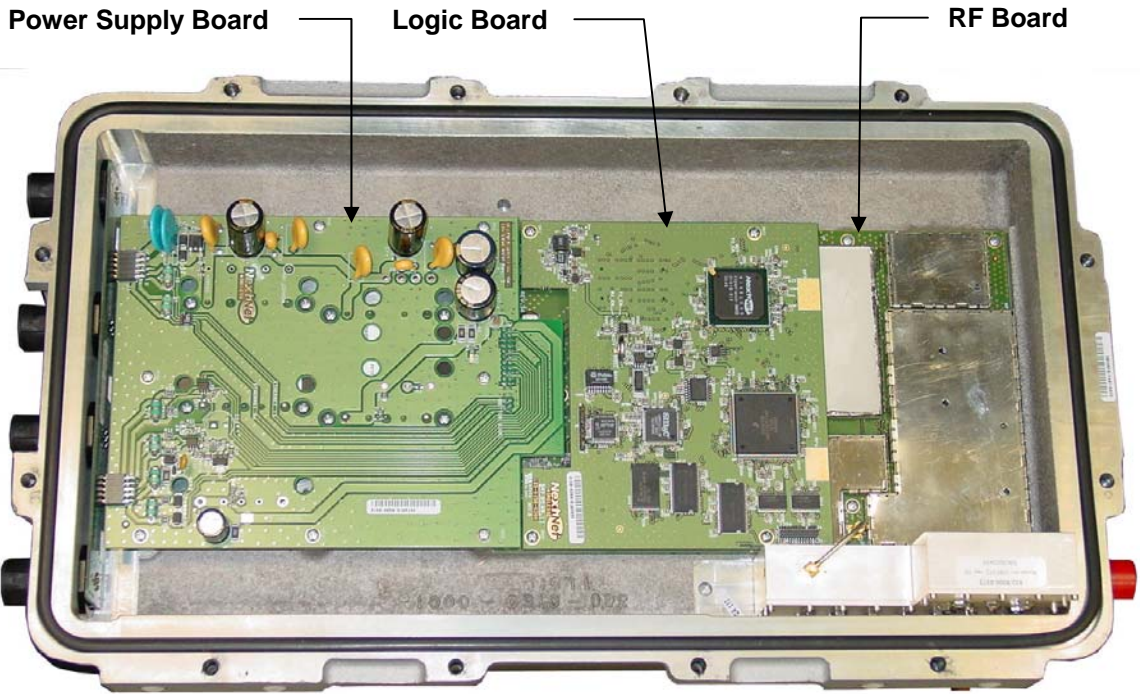
Chassis With Cover Removed
