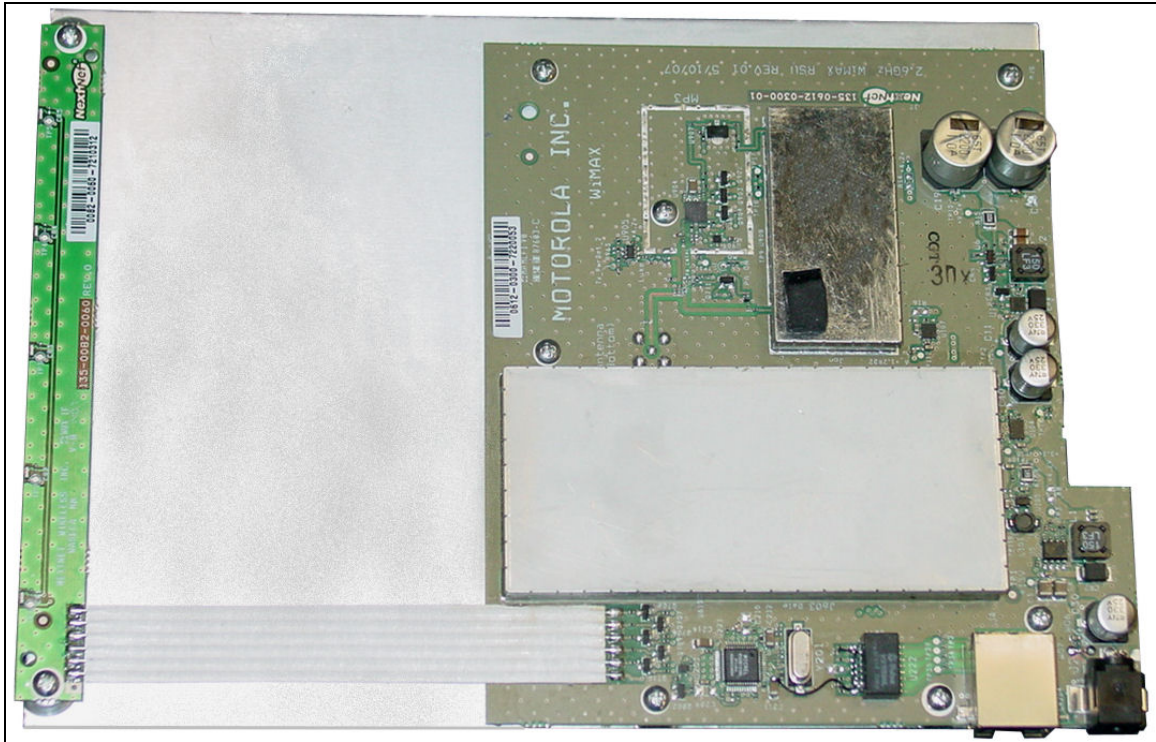
PC Board Component Side View (With Shields Installed)
