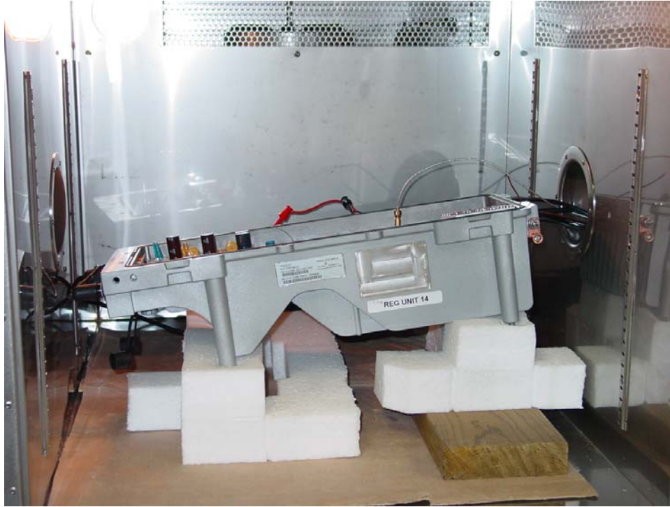
Frequency Stability Test Setup (Inside Chamber)
