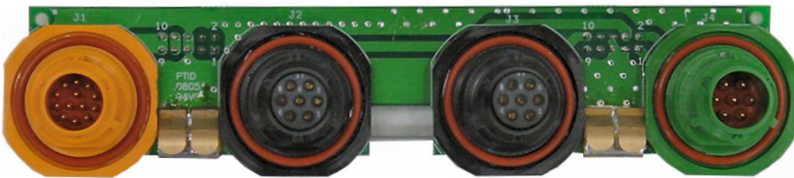
Interconnect Board Front View
