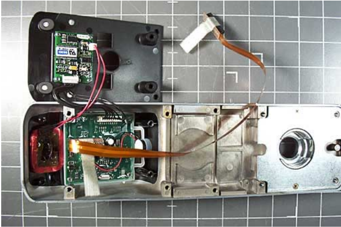
Back of Keypad with Cover Removed
