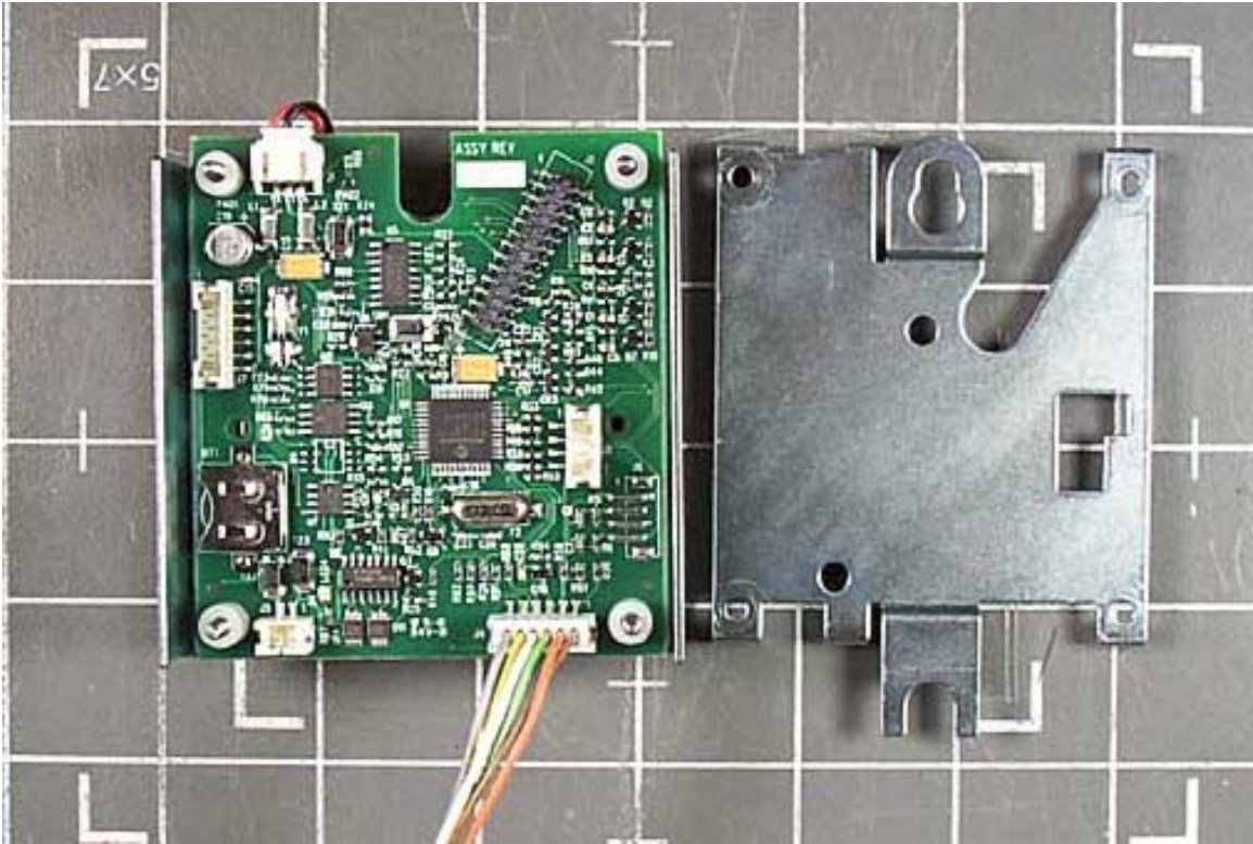
Digital Board – Cover Removed
