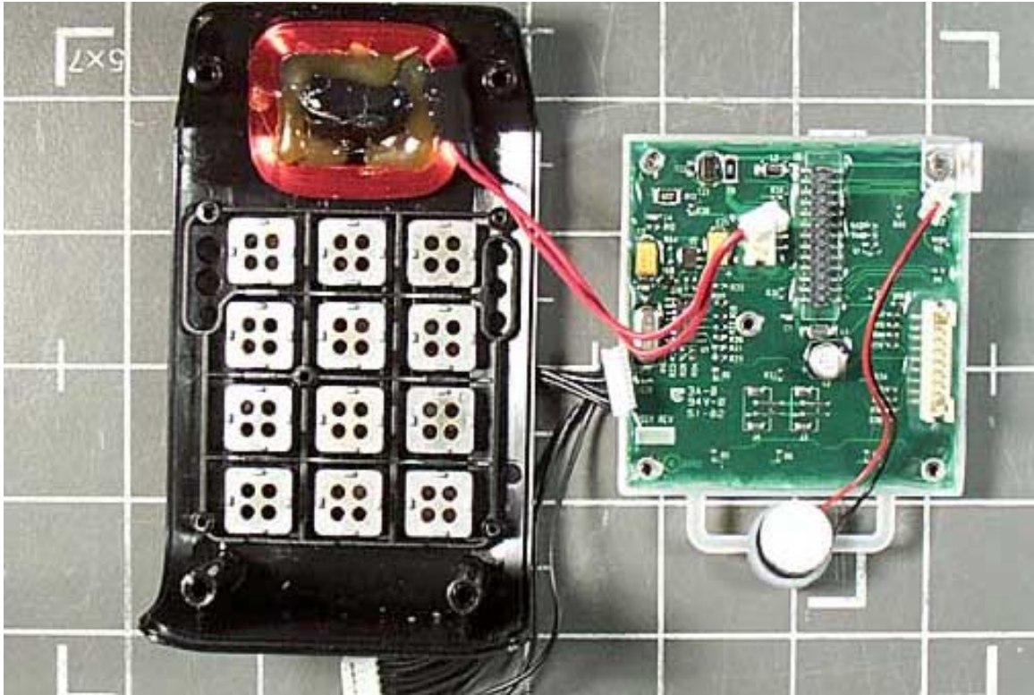
Overall View – Back of Keypad and Large RF PCB
