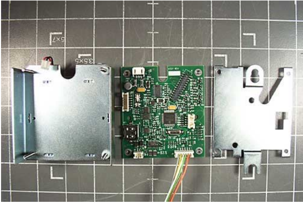
Front Overall View Digital Board - Battery
