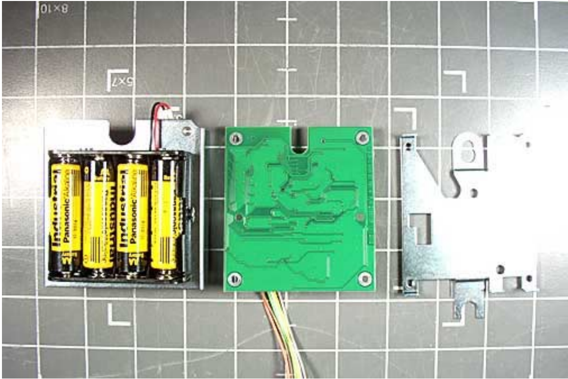
Back Overall View Digital Board - Battery
