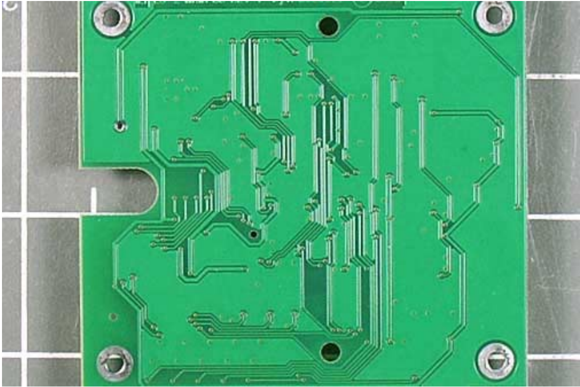
Close-Up of Back of Digital Board
