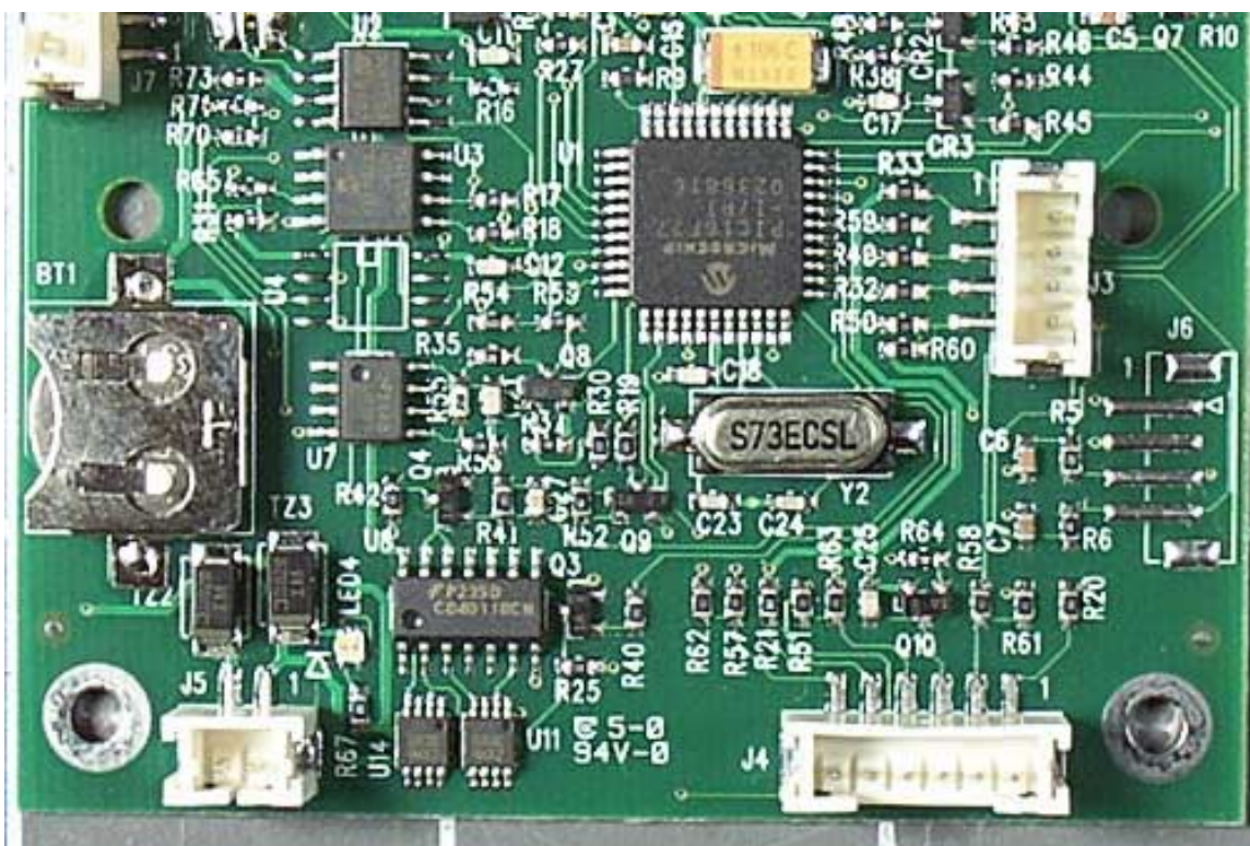
Close-Up of Partial Digital Board – Front Part 1
