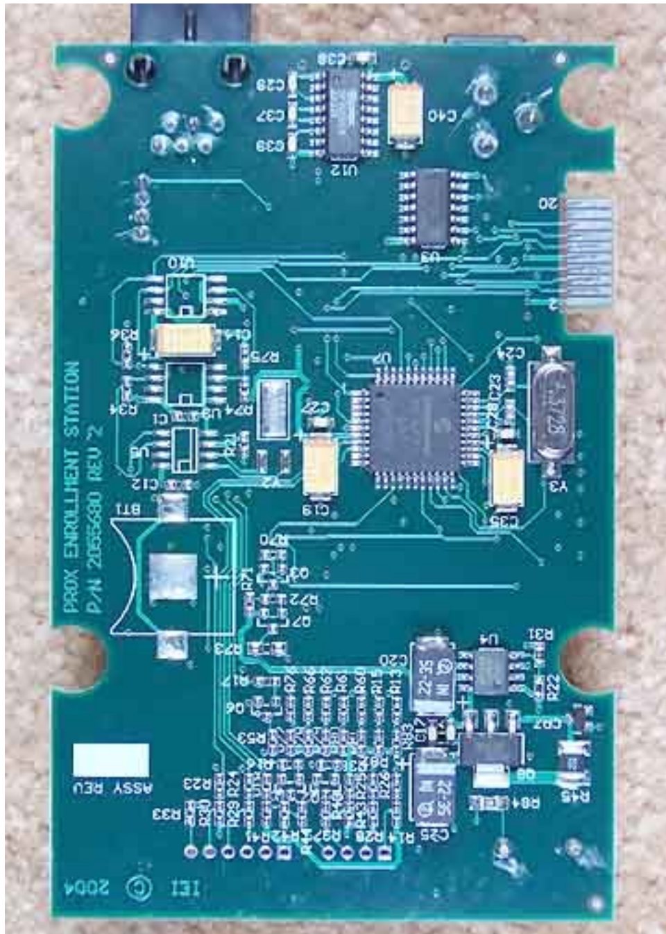
PCB Bottom Closeup
