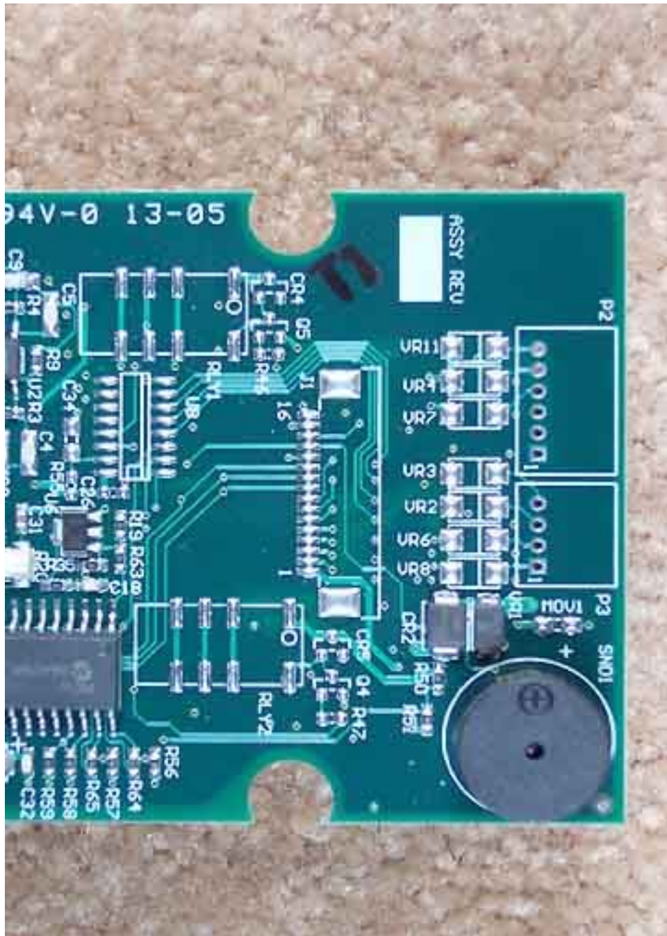
PCB Top Closeup 1
