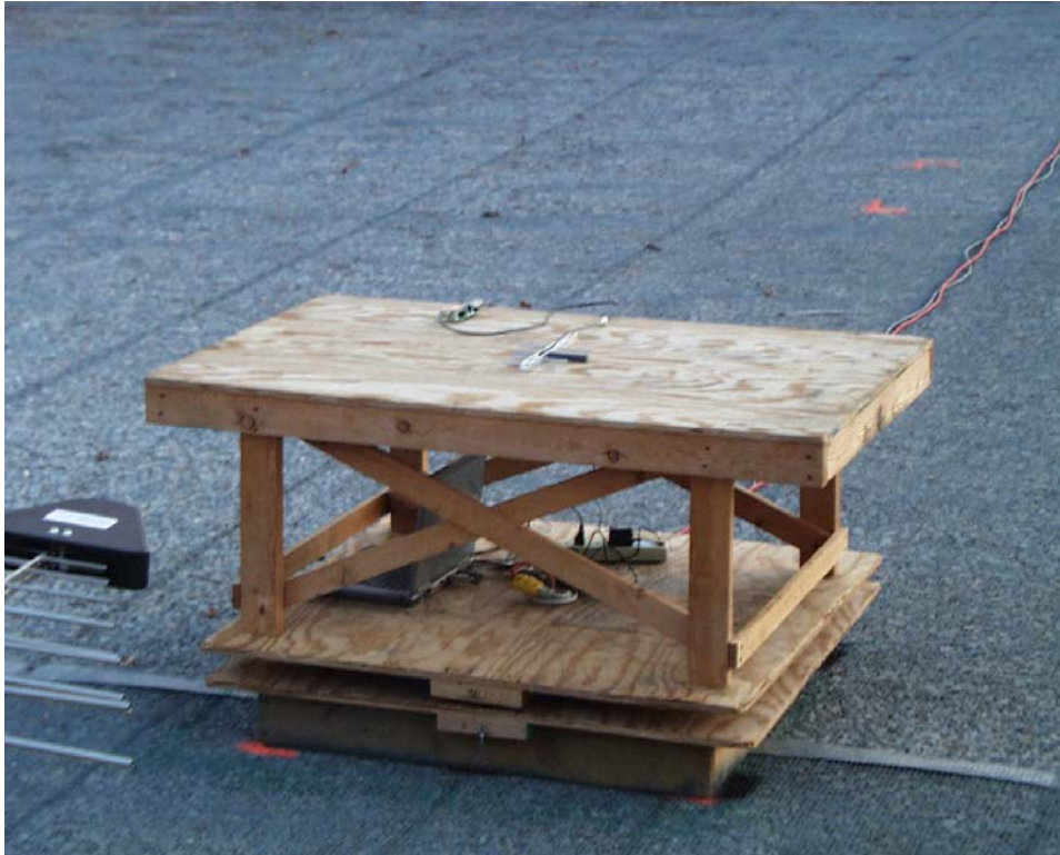
Radiated Emissions Test setup photographs with 6dBi Gain antenna (part number PC904N).
