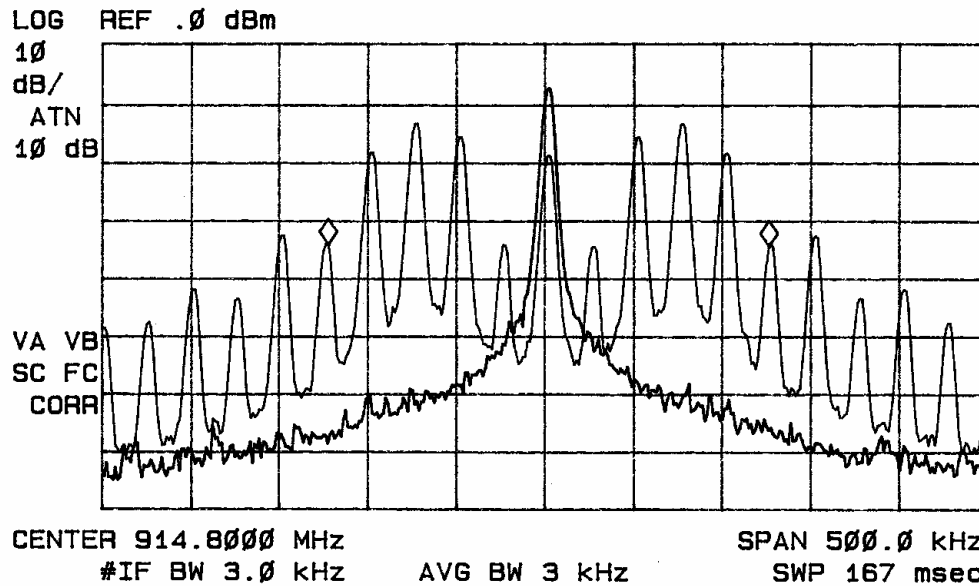
Figure eight 99.5% occupied bandwidth plot
