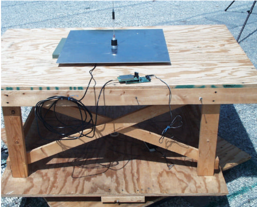
5/8 wave center loaded
