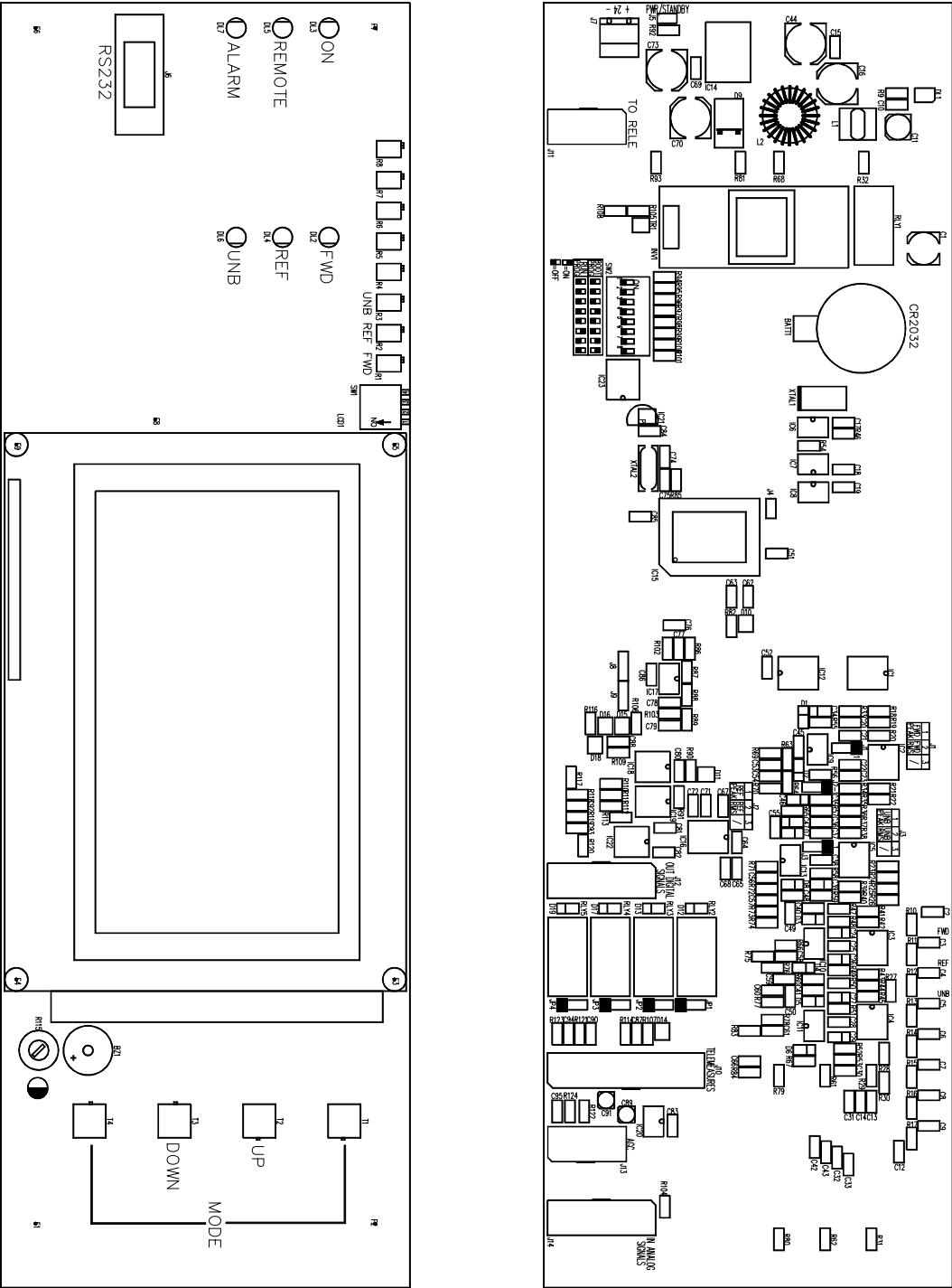
Component layout SCH0239AR0 (Bottom and Top layer)
