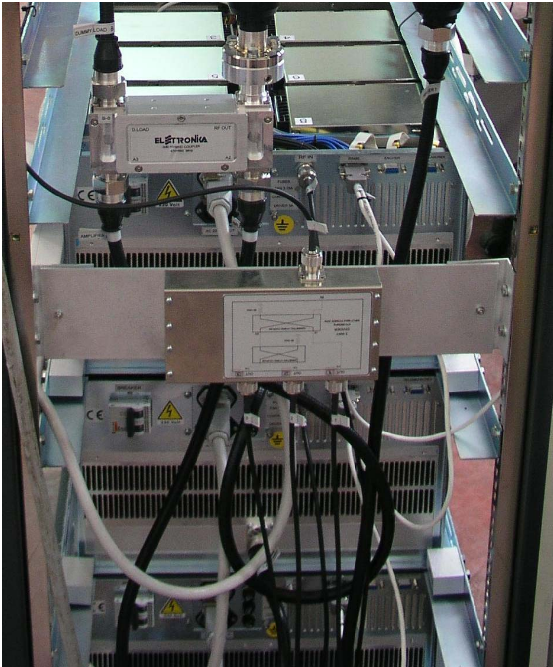
BOTTOM REAR VIEW—DOOR OPEN
