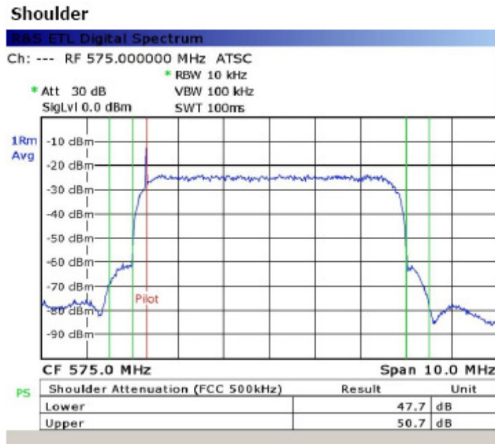
USB and LSB Shoulder Measurement of the desired channel
