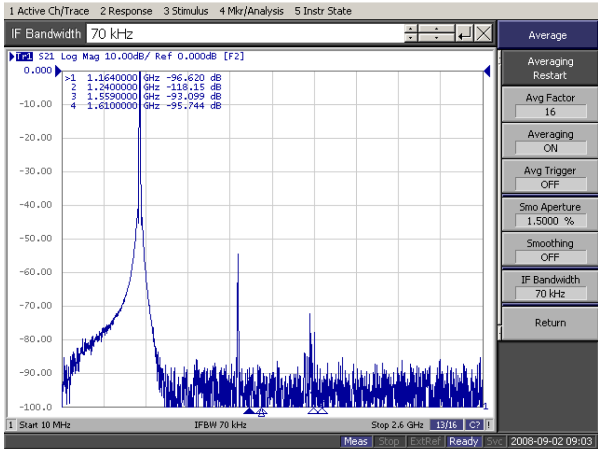
CH23 2 Emission Mask Filter (Combination Bandpass filter and Low Pass Filter Configuration)
