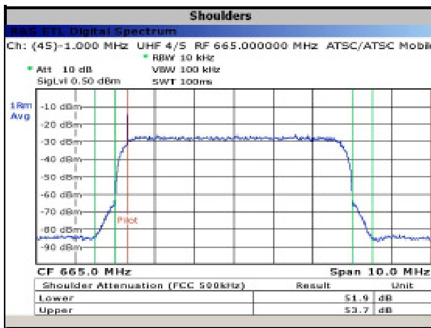
Spectrum shoulder measurement of the desired channel
