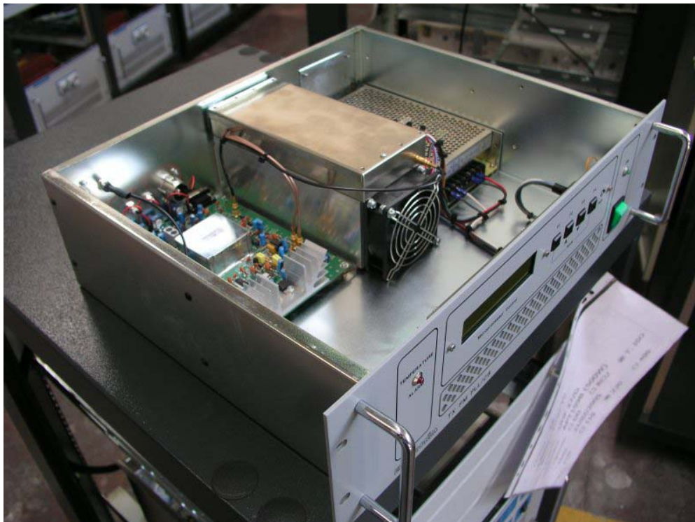
PLLC TOP LEFT VIEW
