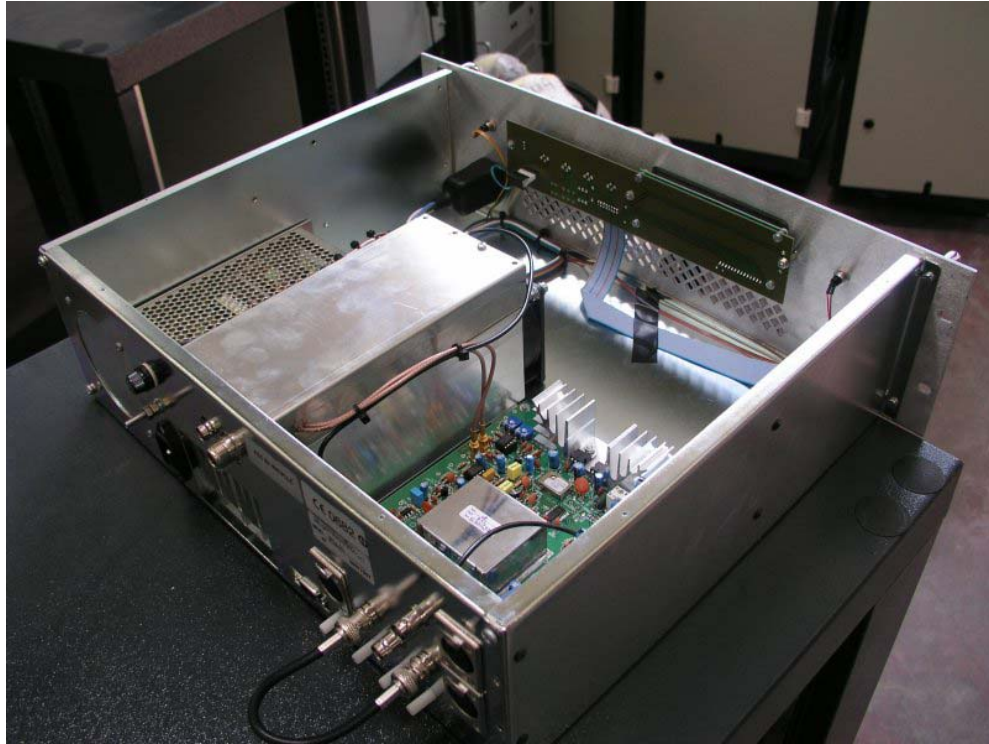
PLLC RIGHT REAR TOP VIEW
