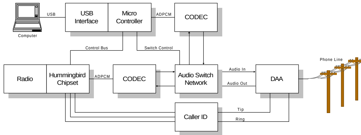
Base Station Block Diagram
