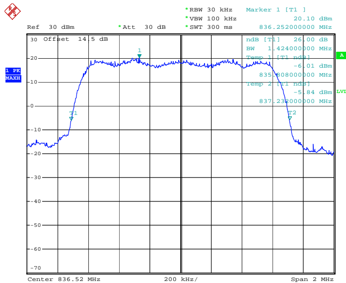
26dB Bandwidth Plot on Channel 384
