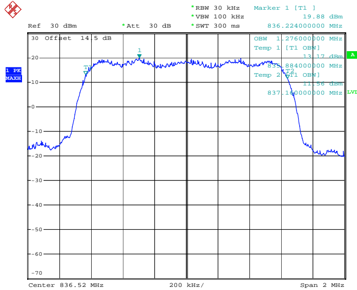
99% Occupied Bandwidth Plot on Channel 384
